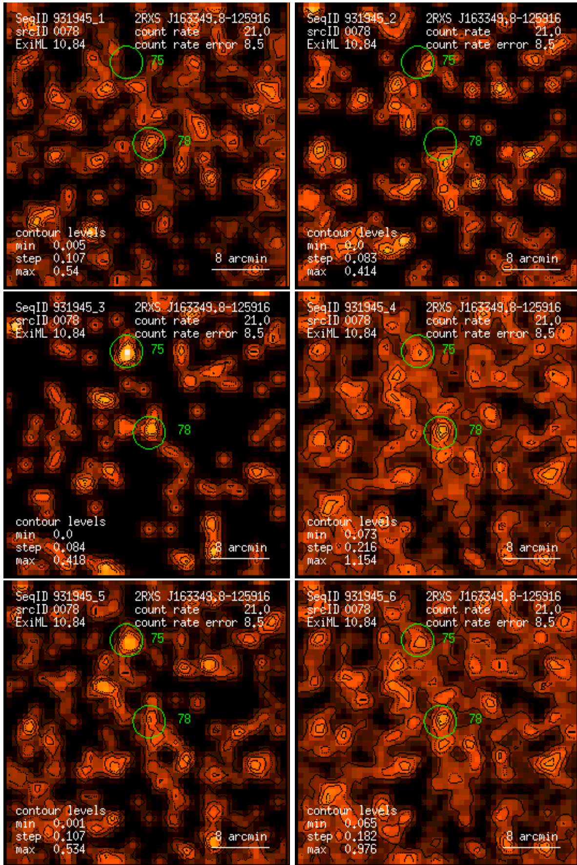
Figure 78: RASS 931945: detection 0078: band rate images, Gaussian filter: (1) PSPPC channels 11 – 41, (2) 52 – 90, (3) 91 – 201, (4) 11 – 235, (5) 52 – 201, (6) 11 – 201. Broad band rates in counts/ks. Band rate contour levels in counts/ks/arcmin 2 .
