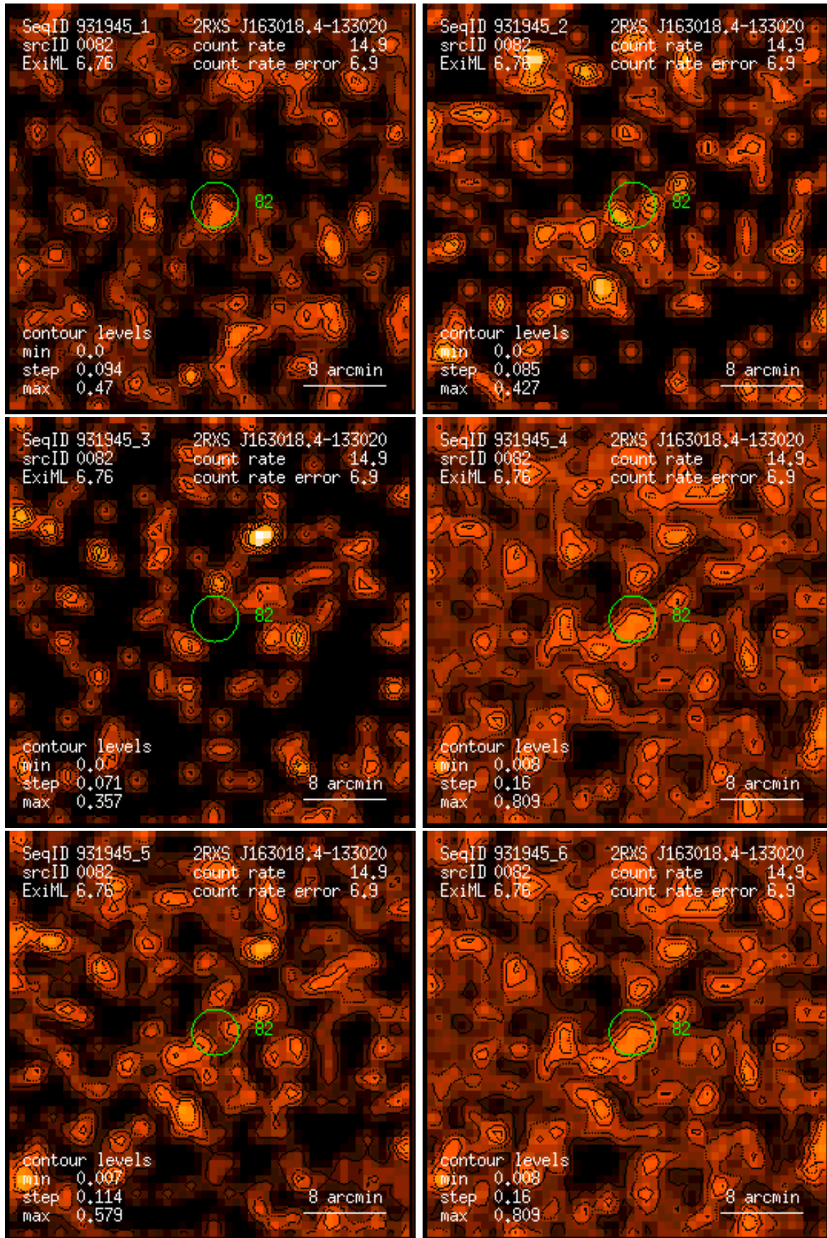
Figure 82: RASS 931945: detection 0082: band rate images, Gaussian filter: (1) PSPC channels 11 – 41, (2) 52 – 90, (3) 91 – 201, (4) 11 – 235, (5) 52 – 201, (6) 11 – 201. Broad band rates in counts/ks. Band rate contour levels in counts/ks/arcmin 2 .
