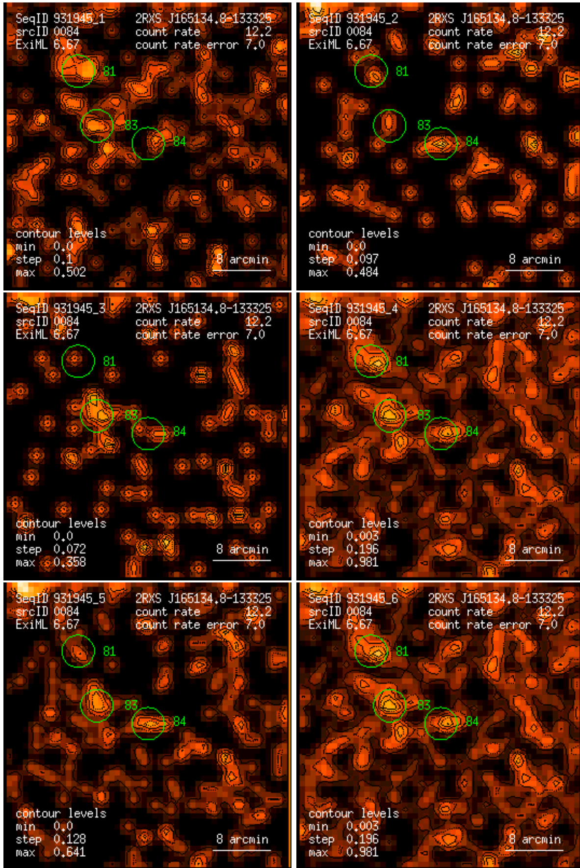
Figure 84: RASS 931945: detection 0084: band rate images, Gaussian filter: (1) PSPC channels 11 – 41, (2) 52 – 90, (3) 91 – 201, (4) 11 – 235, (5) 52 – 201, (6) 11 – 201. Broad band rates in counts/ks. Band rate contour levels in counts/ks/arcmin 2 .
