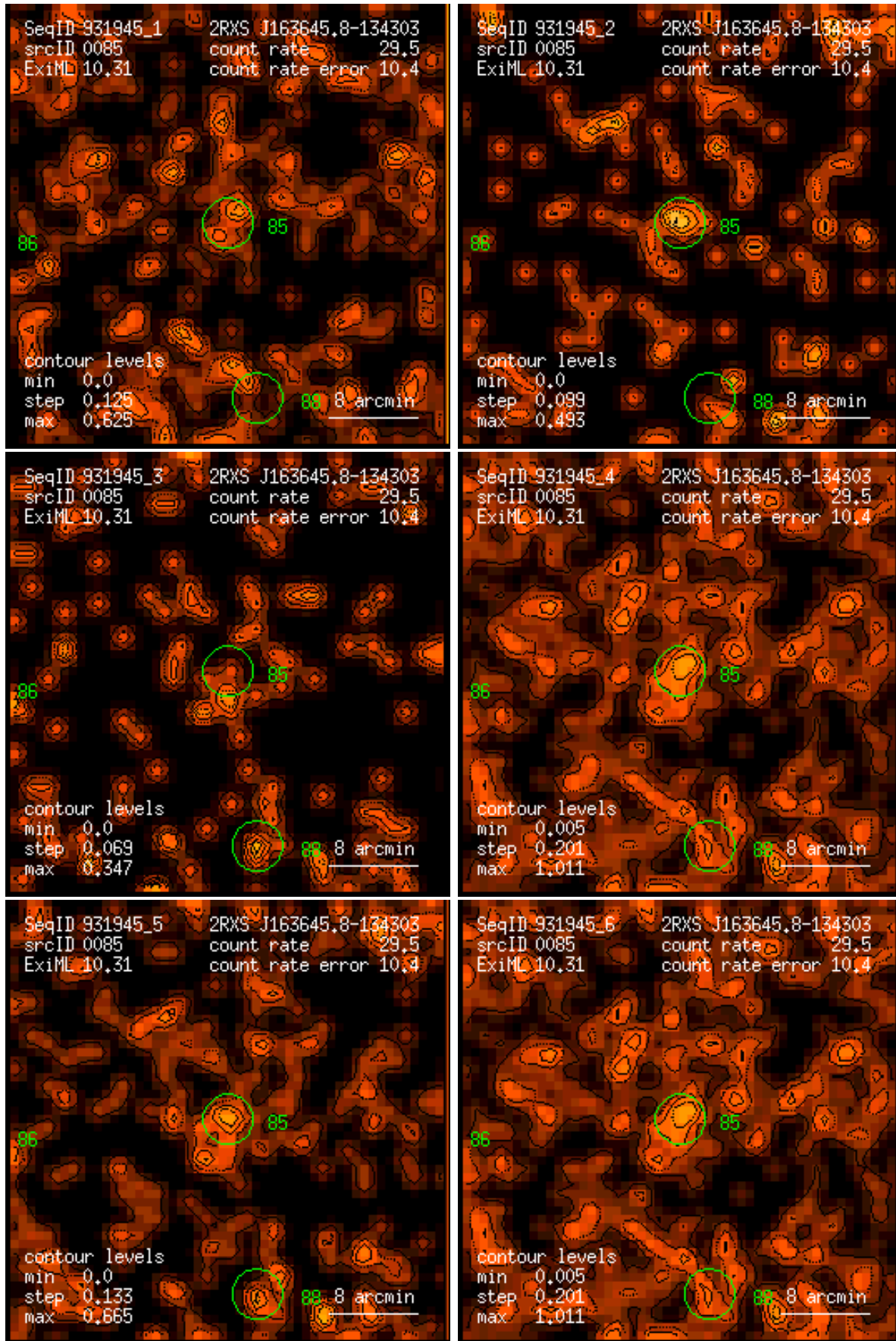
Figure 85: RASS 931945: detection 0085: band rate images, Gaussian filter: (1) PSPC channels 11 – 41, (2) 52 – 90, (3) 91 – 201, (4) 11 – 235, (5) 52 – 201, (6) 11 – 201. Broad band rates in counts/ks. Band rate contour levels in counts/ks/arcmin 2 .
