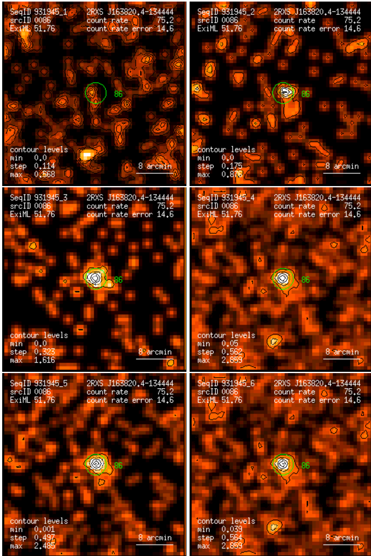
Figure 86: RASS 931945: detection 0086: band rate images, Gaussian filter: (1) PSPC channels 11 – 41, (2) 52 – 90, (3) 91 – 201, (4) 11 – 235, (5) 52 – 201, (6) 11 – 201. Broad band rates in counts/ks. Band rate contour levels in counts/ks/arcmin 2 .
