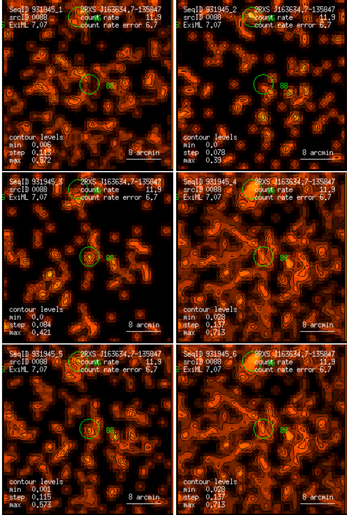
Figure 88: RASS 931945: detection 0088: band rate images, Gaussian filter: (1) PSPC channels 11 – 41, (2) 52 – 90, (3) 91 – 201, (4) 11 – 235, (5) 52 – 201, (6) 11 – 201. Broad band rates in counts/ks. Band rate contour levels in counts/ks/arcmin 2 .
