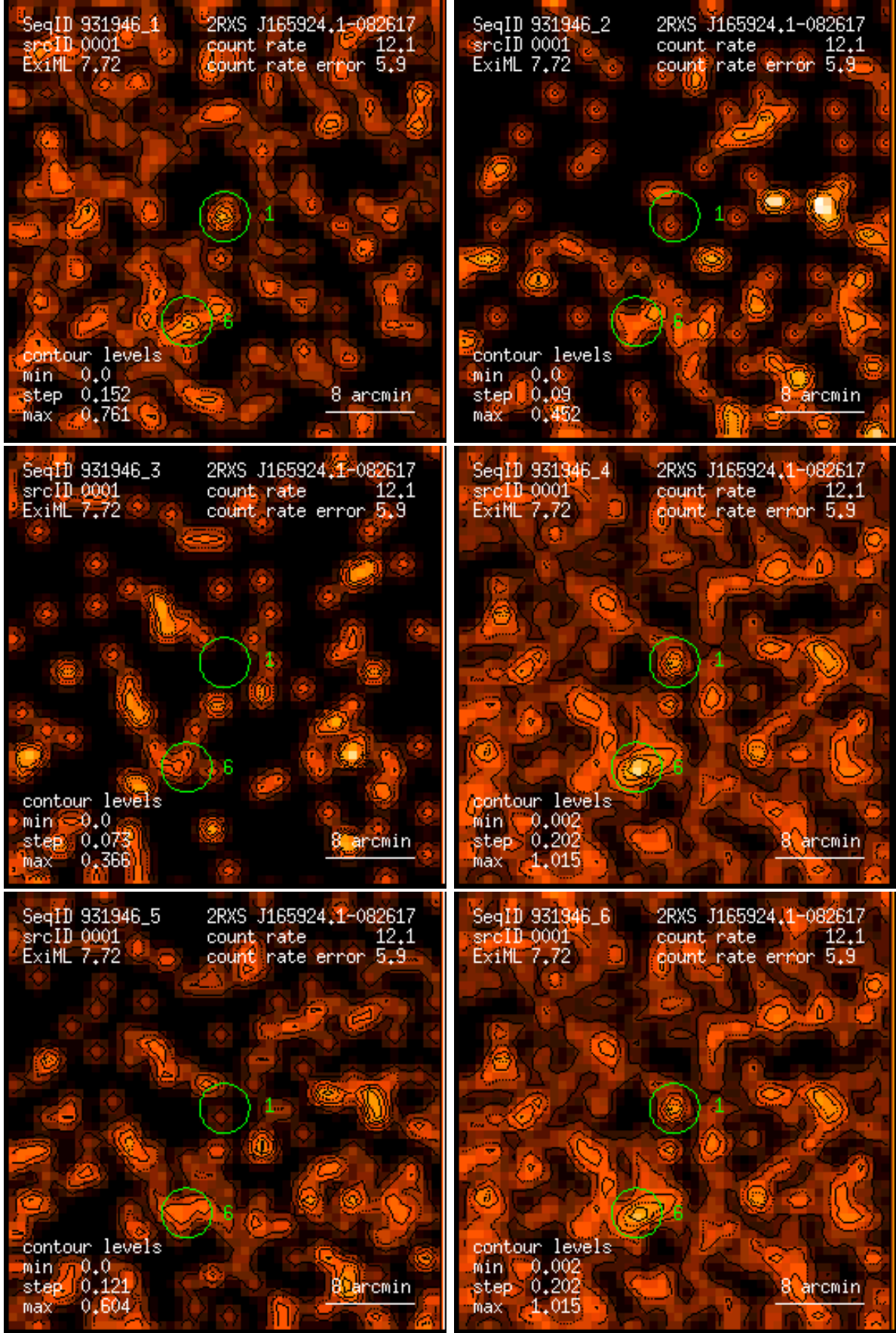
Figure 1: RASS 931946: detection 0001: band rate images, Gaussian filter: (1) PSPC channels 11 – 41, (2) 52 – 90, (3) 91 – 201, (4) 11 – 235, (5) 52 – 201, (6) 11 – 201. Broad band rates in counts/ks. Band rate contour levels in counts/ks/arcmin 2 .
