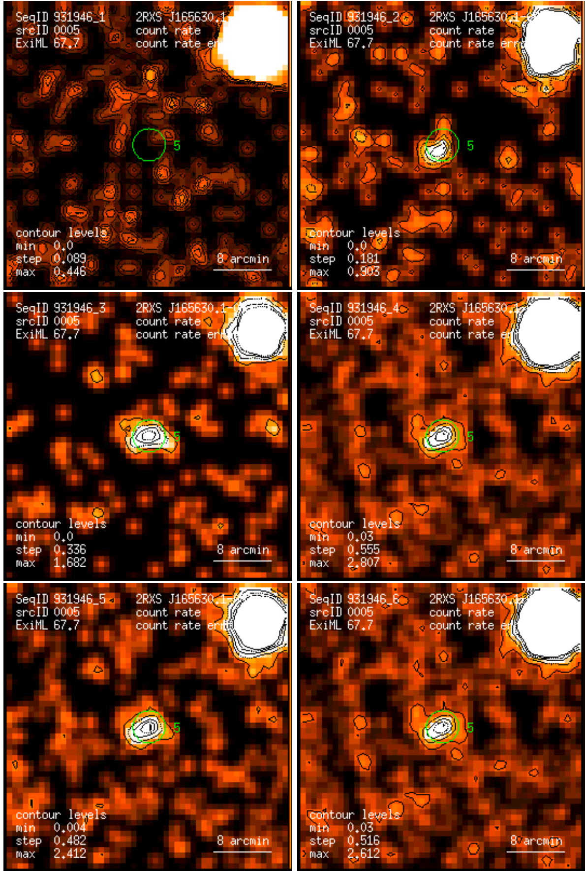
Figure 5: RASS 931946: detection 0005: band rate images, Gaussian filter: (1) PSPC channels 11 – 41, (2) 52 – 90, (3) 91 – 201, (4) 11 – 235, (5) 52 – 201, (6) 11 – 201. Broad band rates in counts/ks. Band rate contour levels in counts/ks/arcmin 2 .
