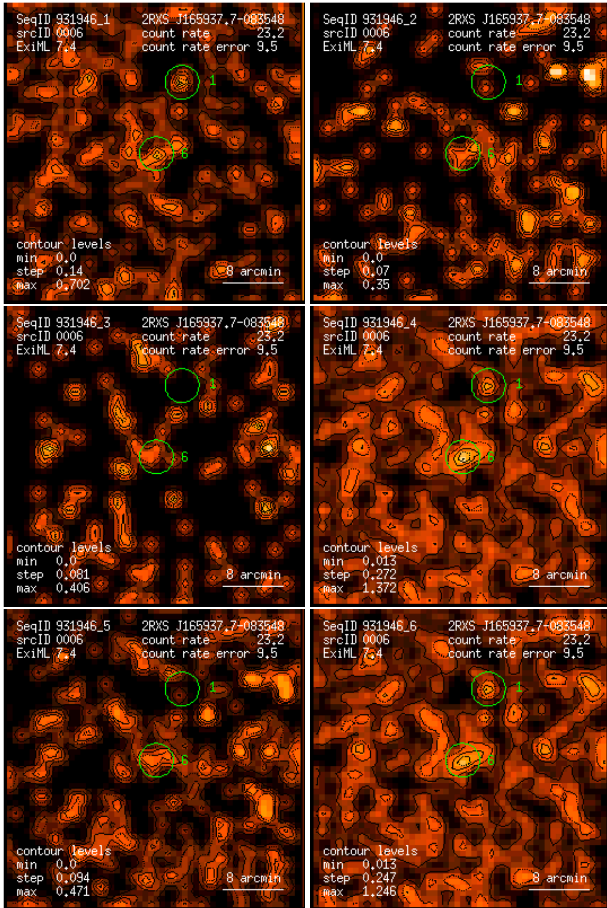
Figure 6: RASS 931946: detection 0006: band rate images, Gaussian filter: (1) PSPC channels 11 – 41, (2) 52 – 90, (3) 91 – 201, (4) 11 – 235, (5) 52 – 201, (6) 11 – 201. Broad band rates in counts/ks. Band rate contour levels in counts/ks/arcmin 2 .
