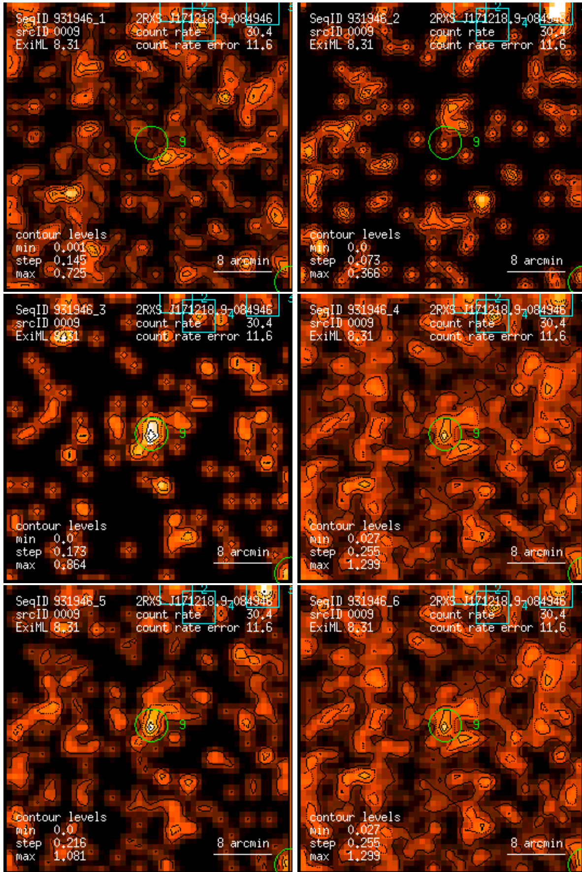
Figure 9: RASS 931946: detection 0009: band rate images, Gaussian filter: (1) PSPC channels 11 – 41, (2) 52 – 90, (3) 91 – 201, (4) 11 – 235, (5) 52 – 201, (6) 11 – 201. Broad band rates in counts/ks. Band rate contour levels in counts/ks/arcmin 2 .
