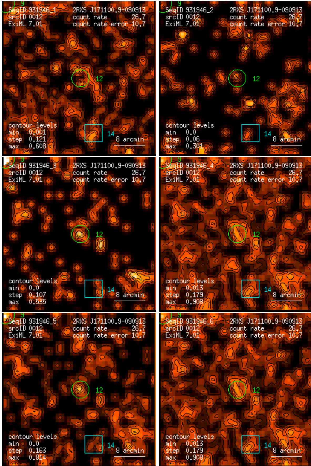
Figure 12: RASS 931946: detection 0012: band rate images, Gaussian filter: (1) PSPC channels 11 – 41, (2) 52 – 90, (3) 91 – 201, (4) 11 – 235, (5) 52 – 201, (6) 11 – 201. Broad band rates in counts/ks. Band rate contour levels in counts/ks/arcmin 2 .
