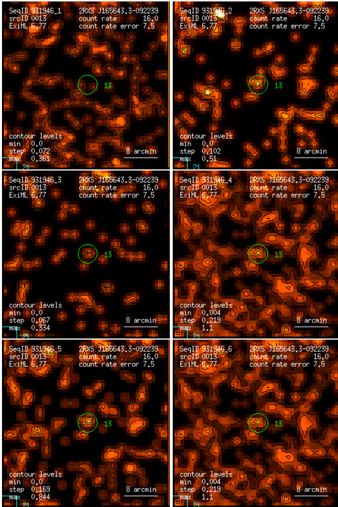
Figure 13: RASS 931946: detection 0013: band rate images, Gaussian filter: (1) PSPC channels 11 – 41, (2) 52 – 90, (3) 91 – 201, (4) 11 – 235, (5) 52 – 201, (6) 11 – 201. Broad band rates in counts/ks. Band rate contour levels in counts/ks/arcmin 2 .
