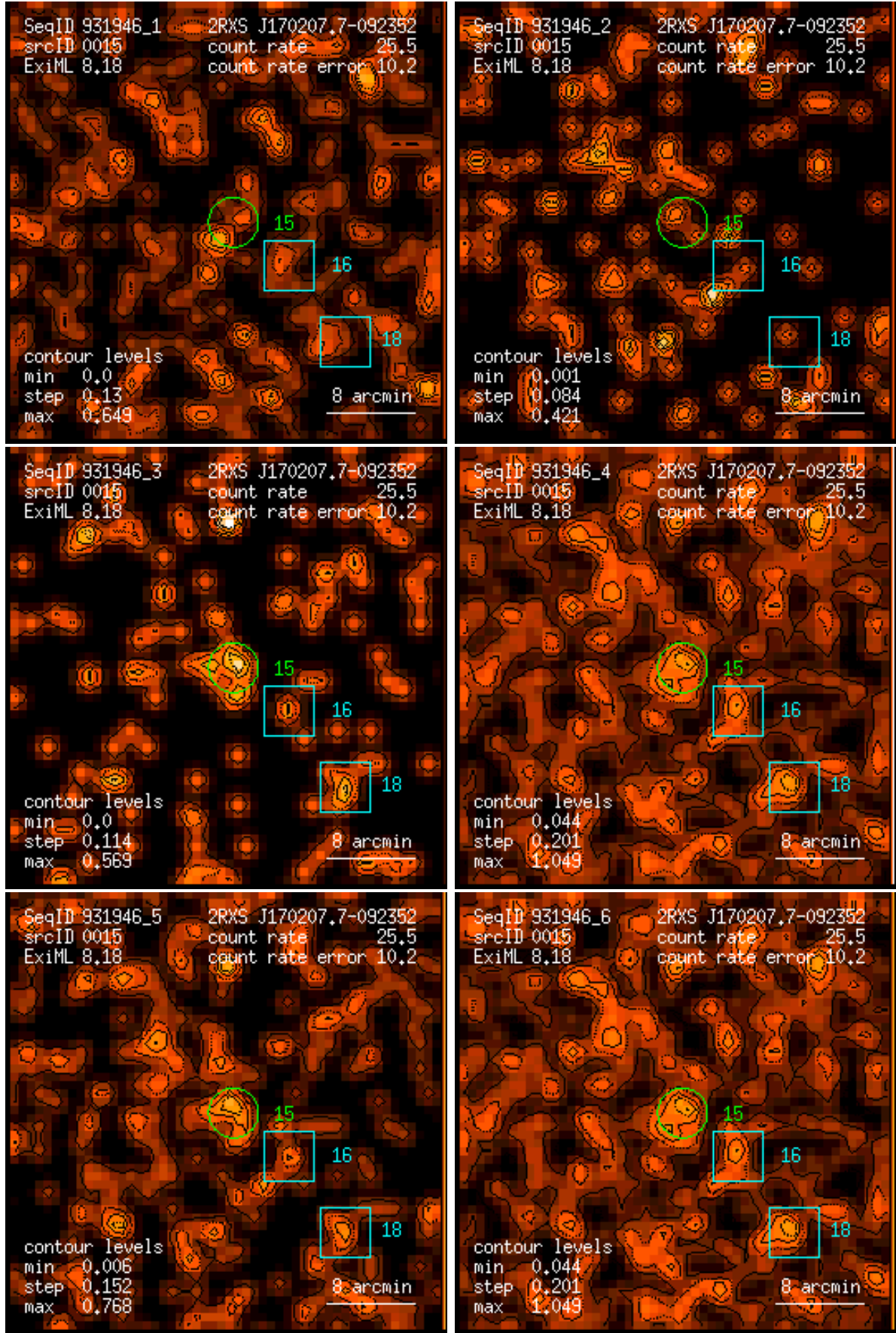
Figure 15: RASS 931946: detection 0015: band rate images, Gaussian filter: (1) PSPC channels 11 – 41, (2) 52 – 90, (3) 91 – 201, (4) 11 – 235, (5) 52 – 201, (6) 11 – 201. Broad band rates in counts/ks. Band rate contour levels in counts/ks/arcmin 2 .
