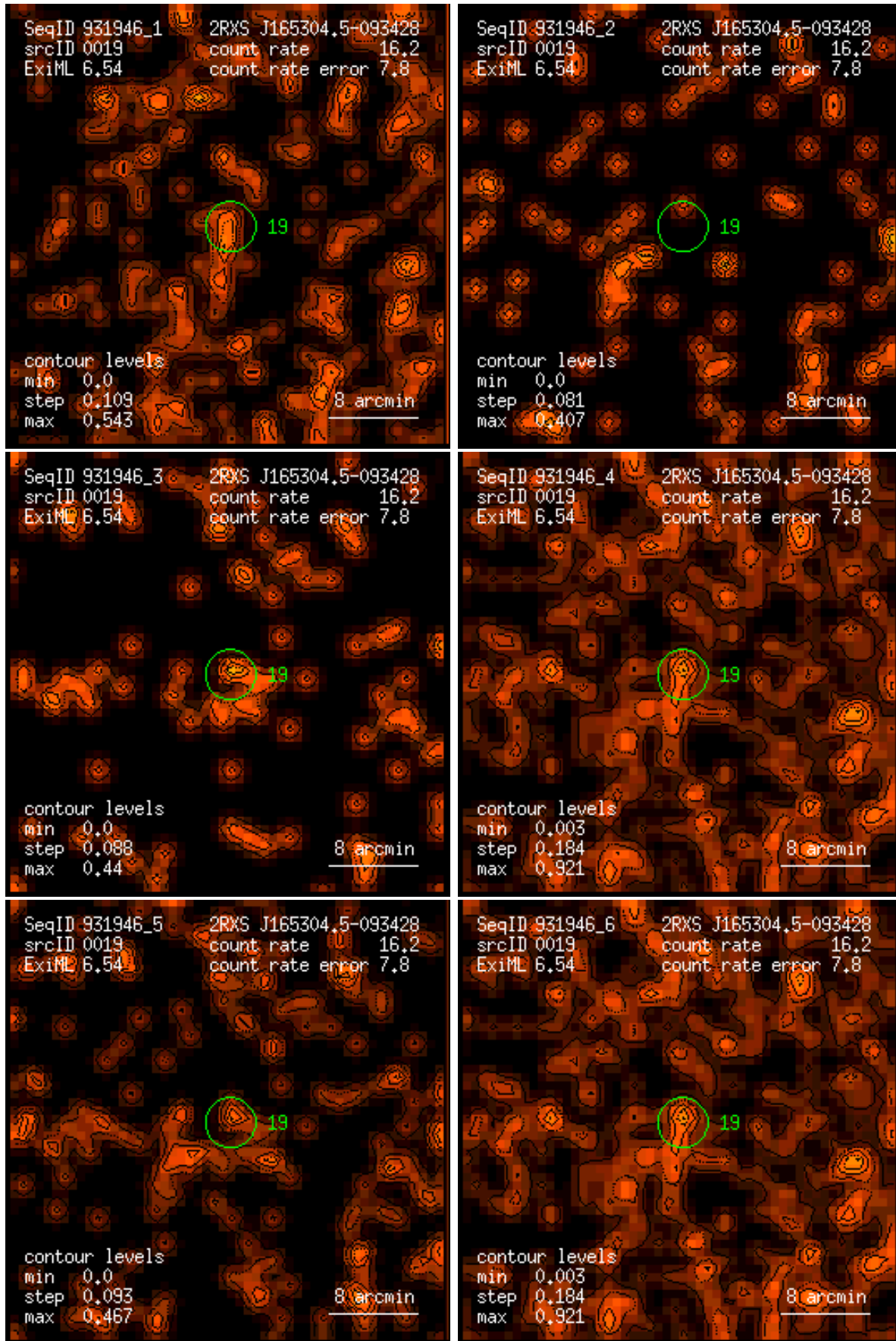
Figure 19: RASS 931946: detection 0019: band rate images, Gaussian filter: (1) PSPC channels 11 – 41, (2) 52 – 90, (3) 91 – 201, (4) 11 – 235, (5) 52 – 201, (6) 11 – 201. Broad band rates in counts/ks. Band rate contour levels in counts/ks/arcmin 2 .
