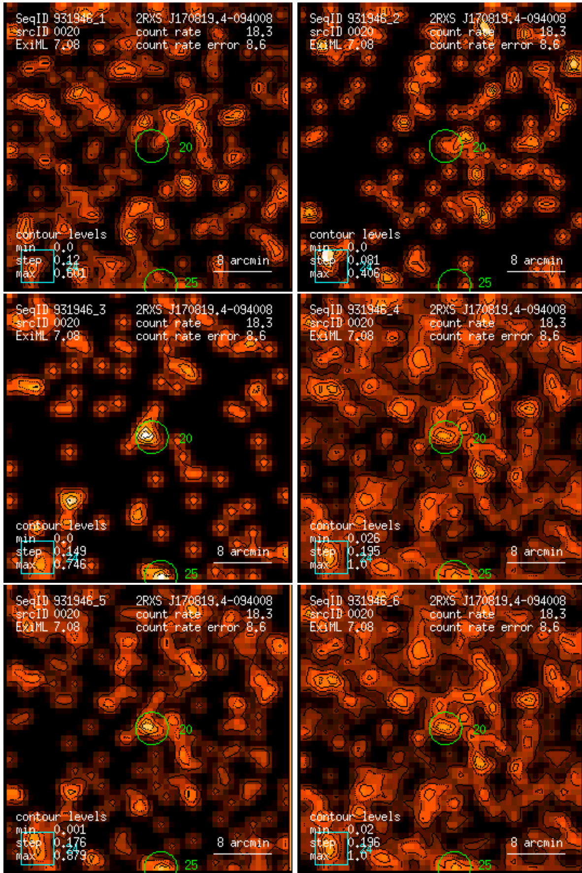
Figure 20: RASS 931946: detection 0020: band rate images, Gaussian filter: (1) PSPC channels 11 – 41, (2) 52 – 90, (3) 91 – 201, (4) 11 – 235, (5) 52 – 201, (6) 11 – 201. Broad band rates in counts/ks. Band rate contour levels in counts/ks/arcmin 2 .
