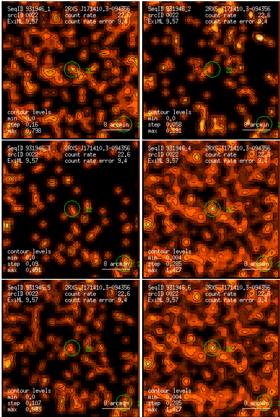
Figure 22: RASS 931946: detection 0022: band rate images, Gaussian filter: (1) PSPC channels 11 – 41, (2) 52 – 90, (3) 91 – 201, (4) 11 – 235, (5) 52 – 201, (6) 11 – 201. Broad band rates in counts/ks. Band rate contour levels in counts/ks/arcmin 2 .
