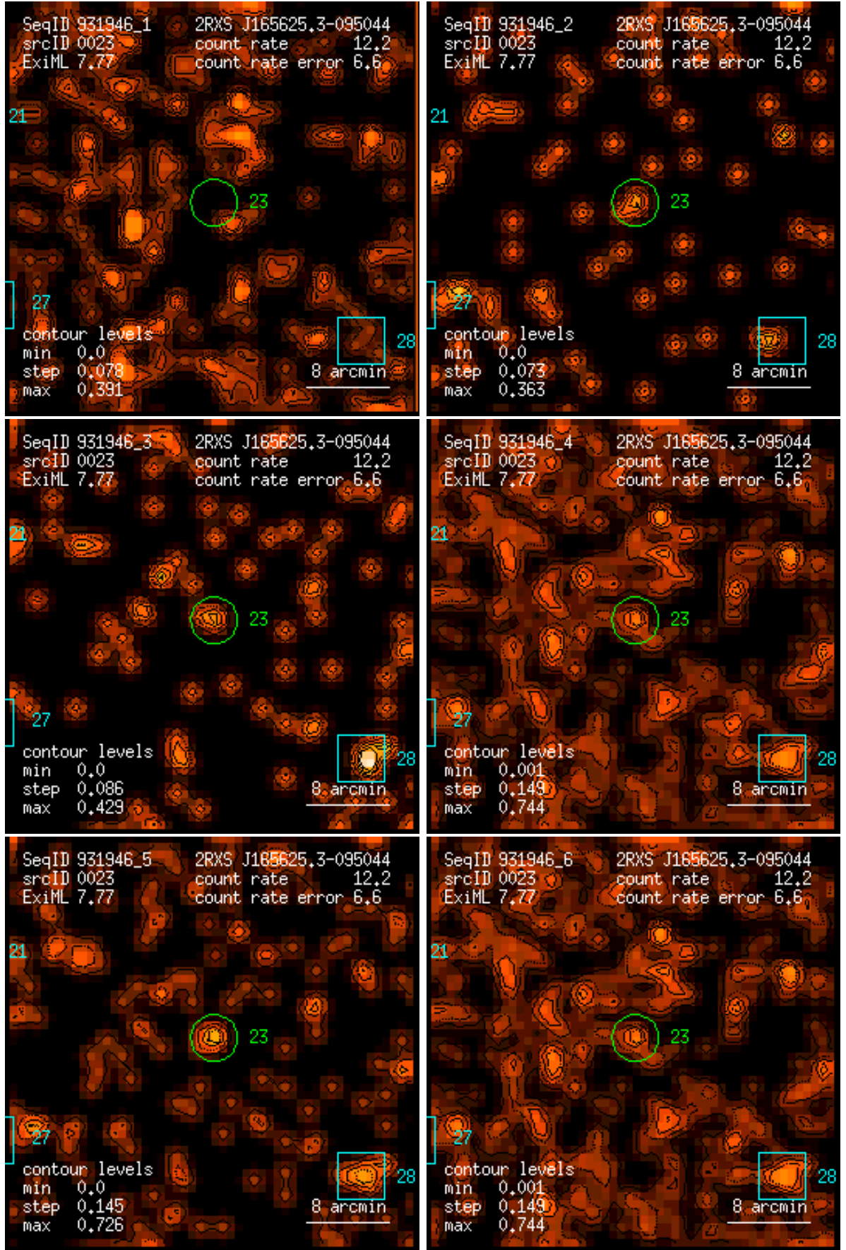
Figure 23: RASS 931946: detection 0023: band rate images, Gaussian filter: (1) PSPC channels 11 – 41, (2) 52 – 90, (3) 91 – 201, (4) 11 – 235, (5) 52 – 201, (6) 11 – 201. Broad band rates in counts/ks. Band rate contour levels in counts/ks/arcmin 2 .
