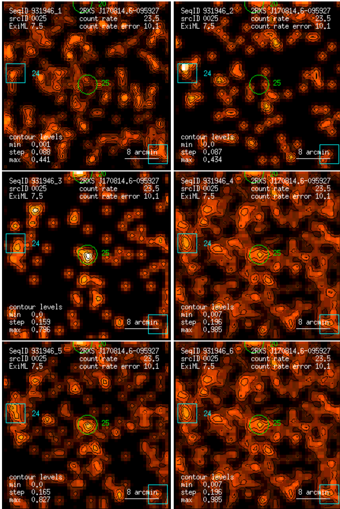
Figure 25: RASS 931946: detection 0025: band rate images, Gaussian filter: (1) PSPC channels 11 – 41, (2) 52 – 90, (3) 91 – 201, (4) 11 – 235, (5) 52 – 201, (6) 11 – 201. Broad band rates in counts/ks. Band rate contour levels in counts/ks/arcmin 2 .
