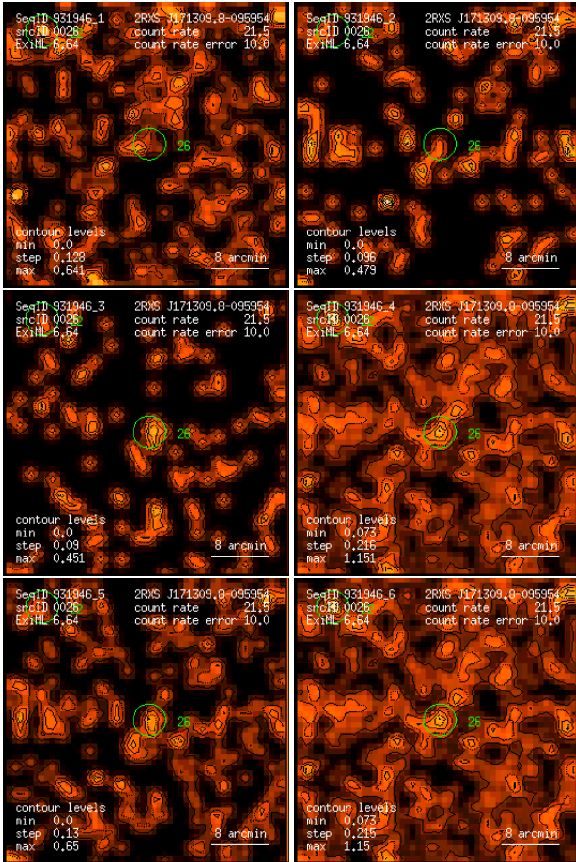
Figure 26: RASS 931946: detection 0026: band rate images, Gaussian filter: (1) PSPC channels 11 – 41, (2) 52 – 90, (3) 91 – 201, (4) 11 – 235, (5) 52 – 201, (6) 11 – 201. Broad band rates in counts/ks. Band rate contour levels in counts/ks/arcmin 2 .
