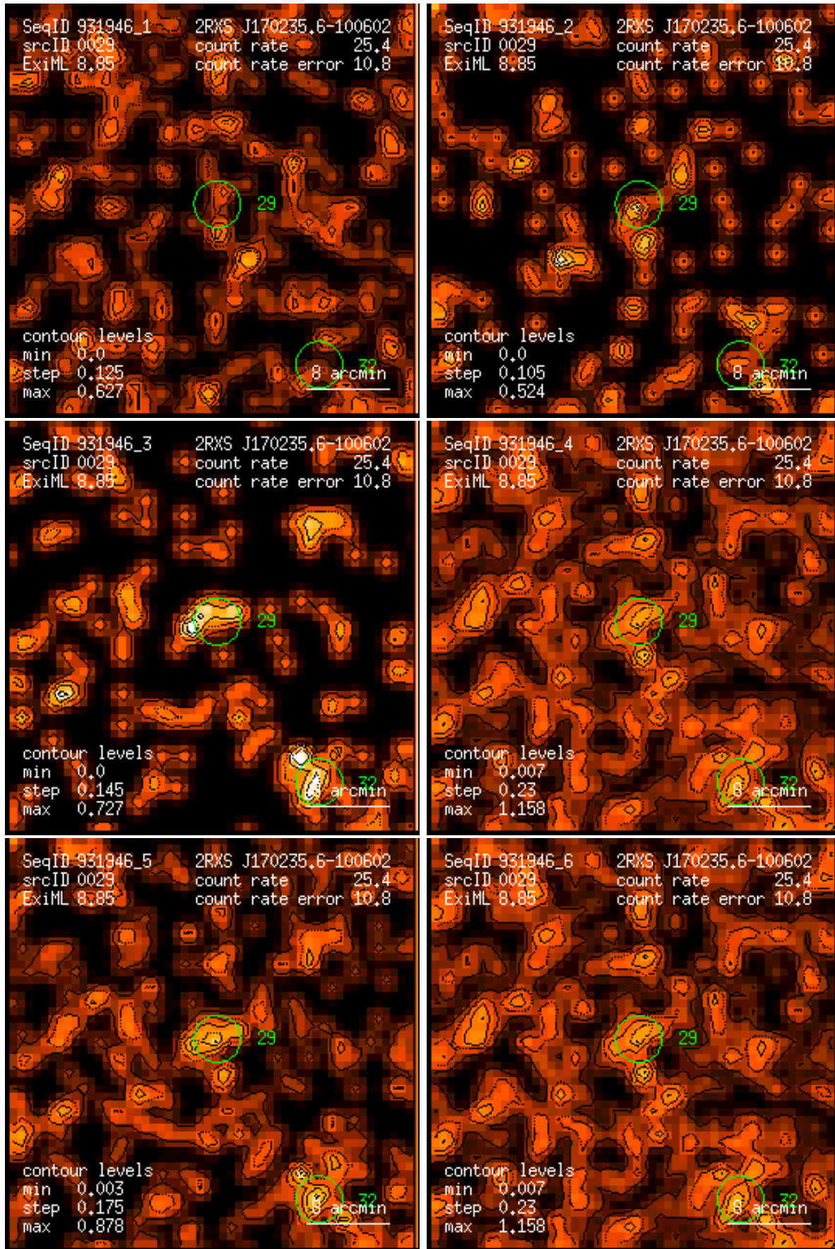
Figure 29: RASS 931946: detection 0029: band rate images, Gaussian filter: (1) PSPC channels 11 – 41, (2) 52 – 90, (3) 91 – 201, (4) 11 – 235, (5) 52 – 201, (6) 11 – 201. Broad band rates in counts/ks. Band rate contour levels in counts/ks/arcmin 2 .
