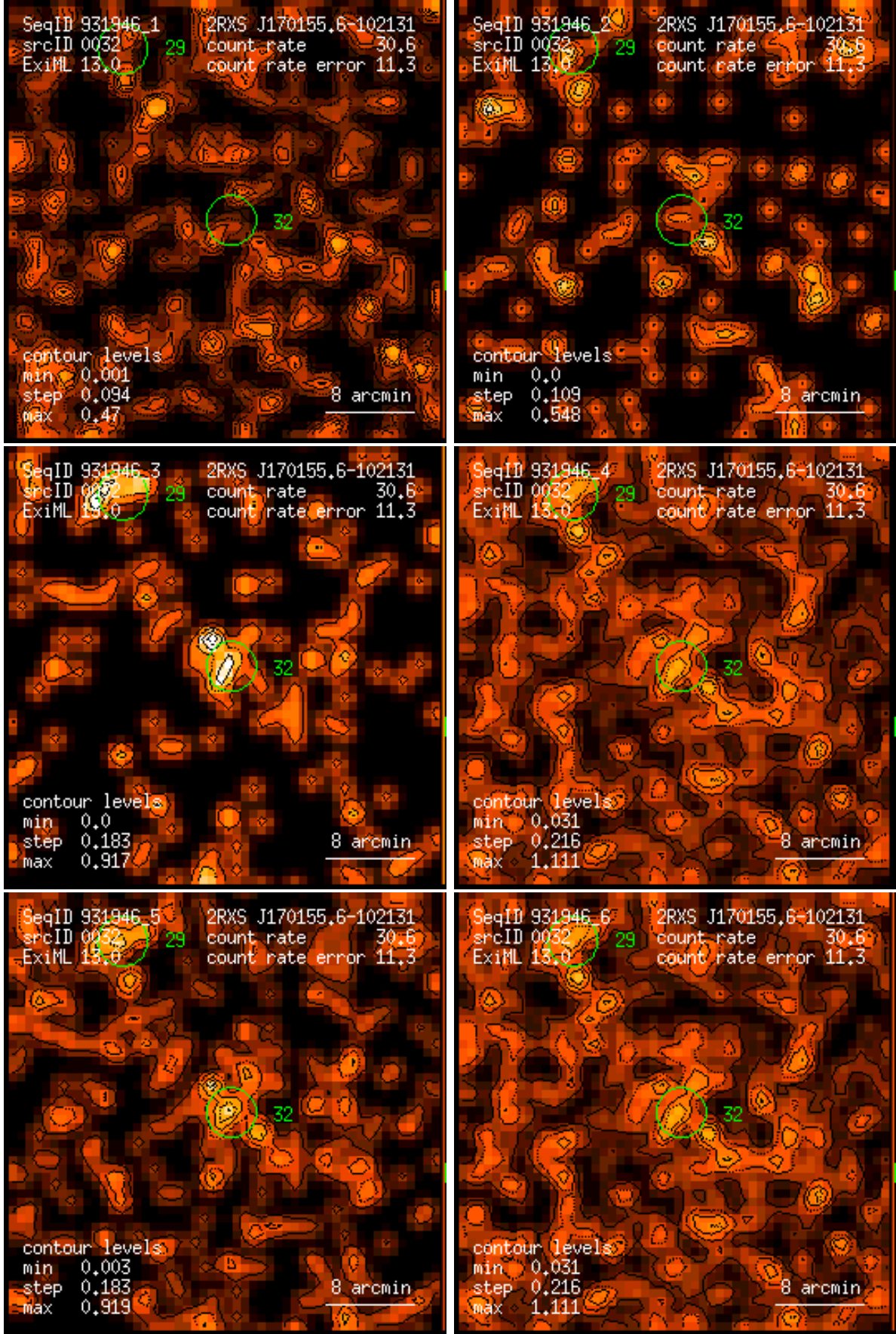
Figure 32: RASS 931946: detection 0032: band rate images, Gaussian filter: (1) PSPC channels 11 – 41, (2) 52 – 90, (3) 91 – 201, (4) 11 – 235, (5) 52 – 201, (6) 11 – 201. Broad band rates in counts/ks. Band rate contour levels in counts/ks/arcmin 2 .
