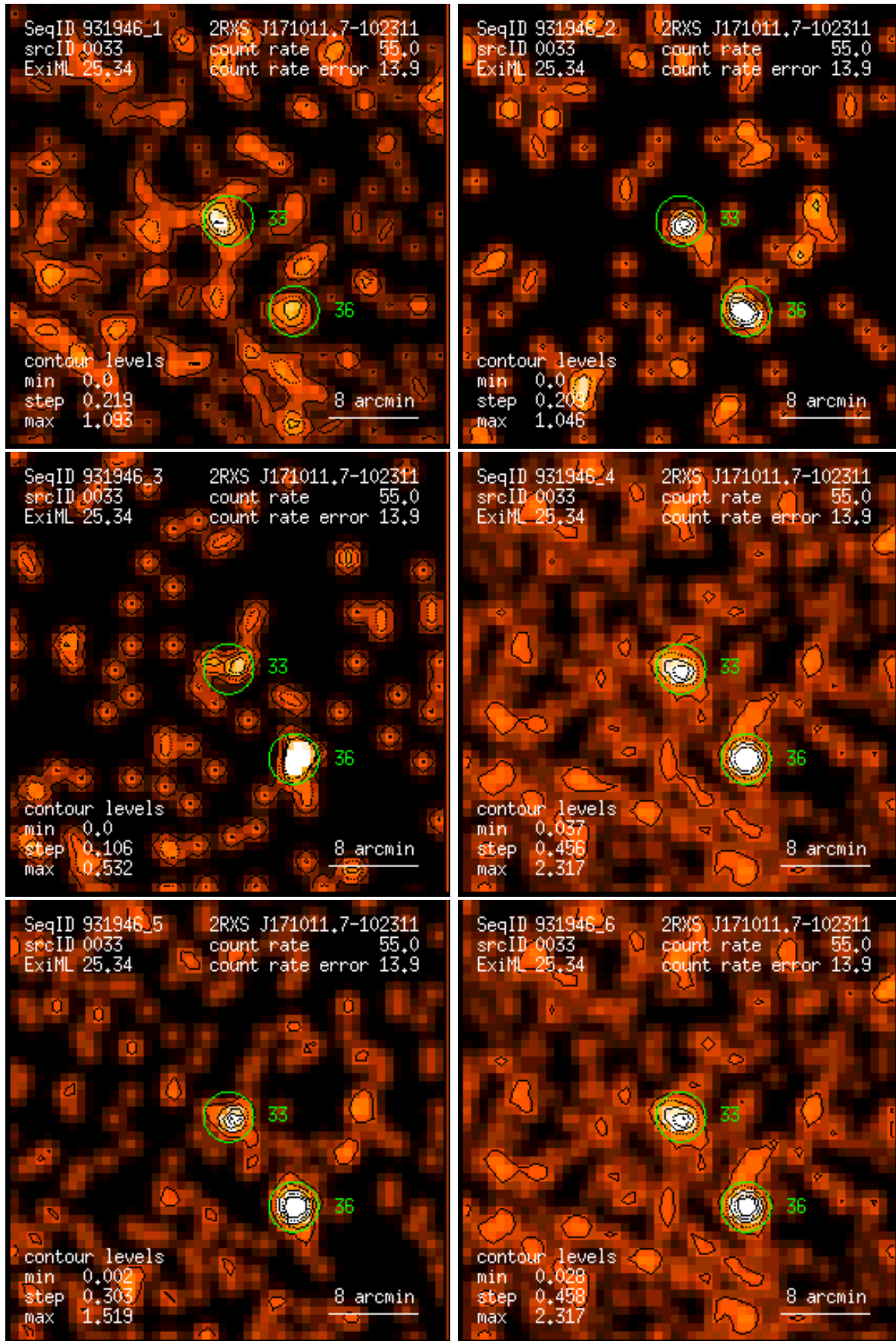
Figure 33: RASS 931946: detection 0033: band rate images, Gaussian filter: (1) PSPC channels 11 – 41, (2) 52 – 90, (3) 91 – 201, (4) 11 – 235, (5) 52 – 201, (6) 11 – 201. Broad band rates in counts/ks. Band rate contour levels in counts/ks/arcmin 2 .
