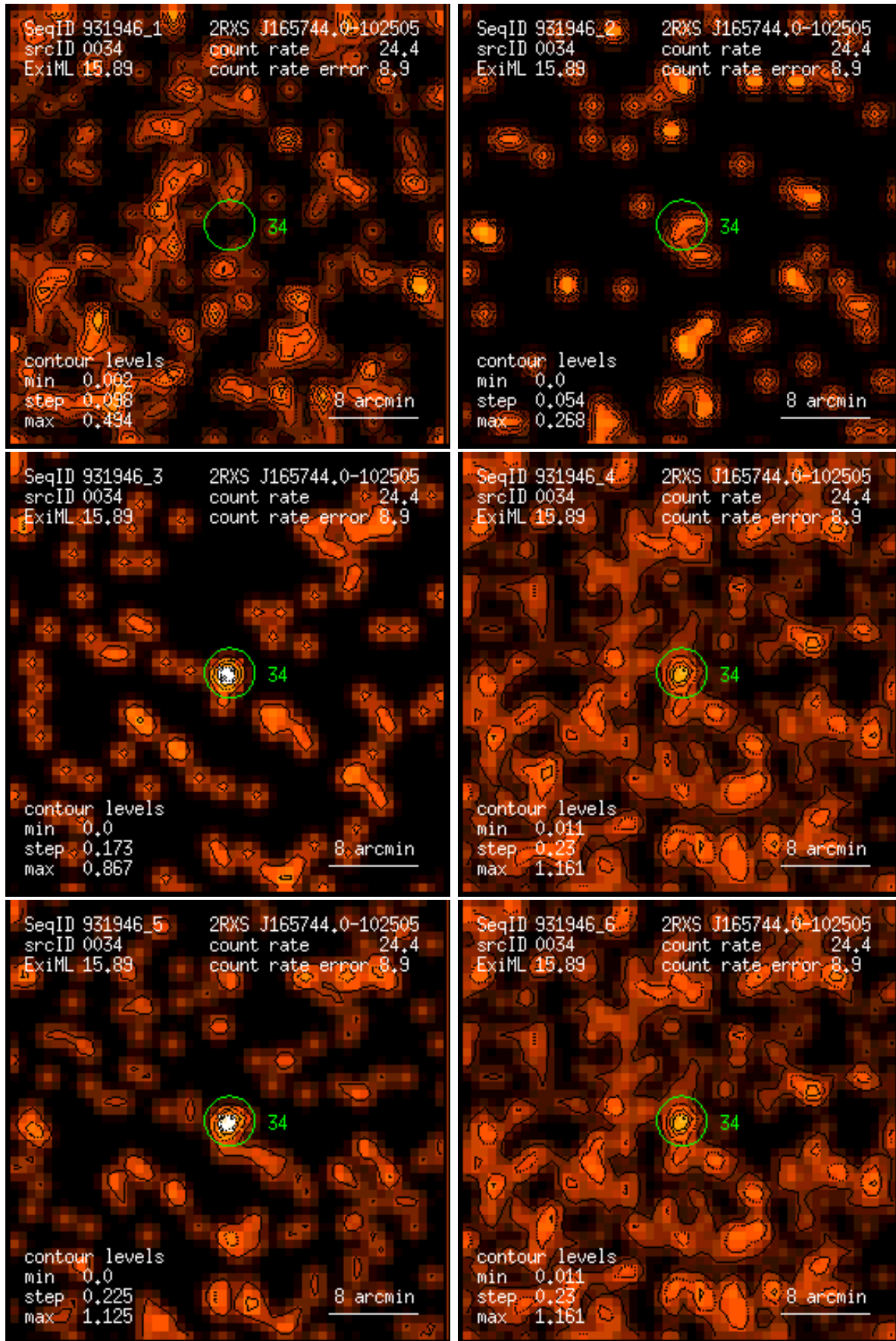
Figure 34: RASS 931946: detection 0034: band rate images, Gaussian filter: (1) PSPC channels 11 – 41, (2) 52 – 90, (3) 91 – 201, (4) 11 – 235, (5) 52 – 201, (6) 11 – 201. Broad band rates in counts/ks. Band rate contour levels in counts/ks/arcmin 2 .
