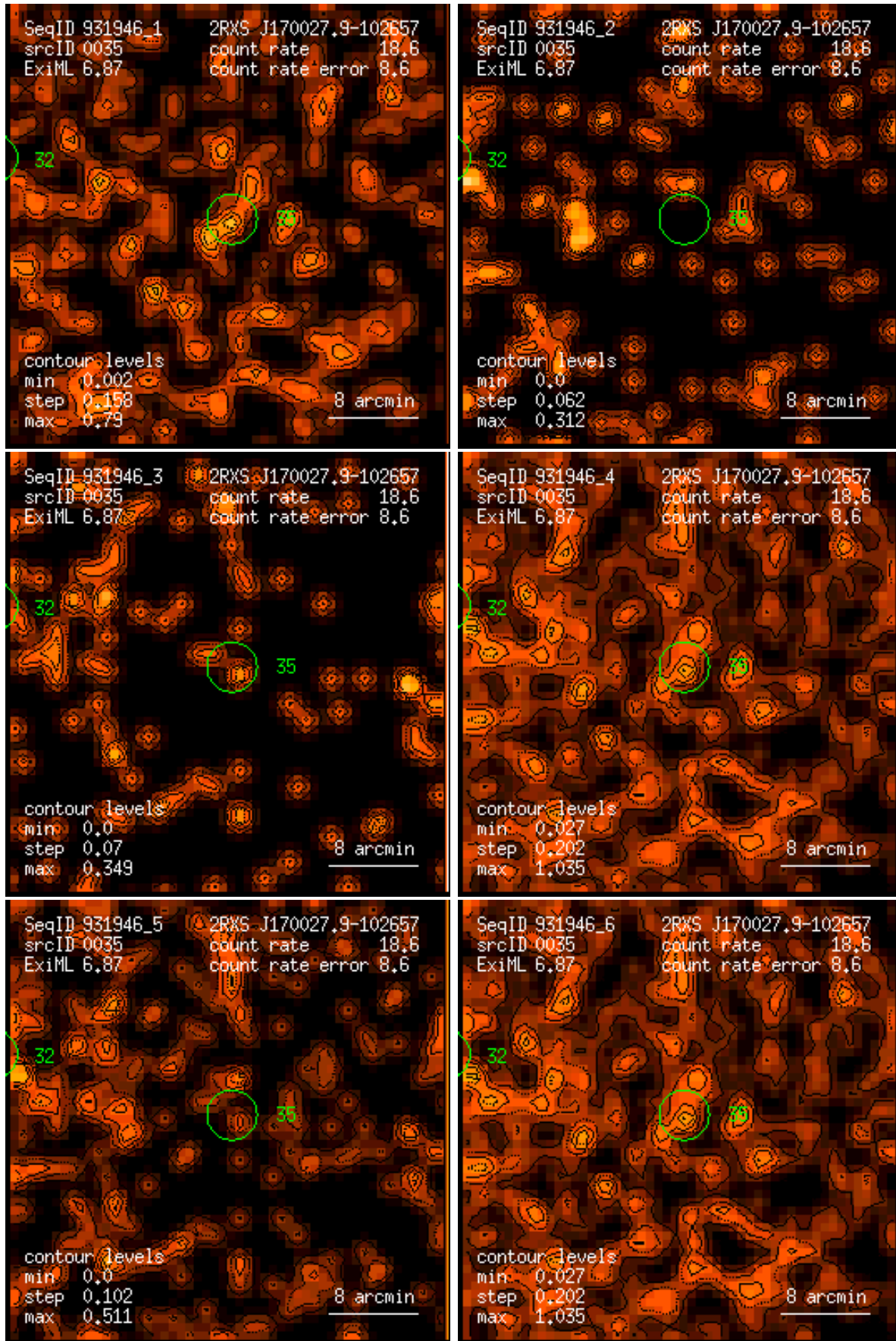
Figure 35: RASS 931946: detection 0035: band rate images, Gaussian filter: (1) PSPC channels 11 – 41, (2) 52 – 90, (3) 91 – 201, (4) 11 – 235, (5) 52 – 201, (6) 11 – 201. Broad band rates in counts/ks. Band rate contour levels in counts/ks/arcmin 2 .
