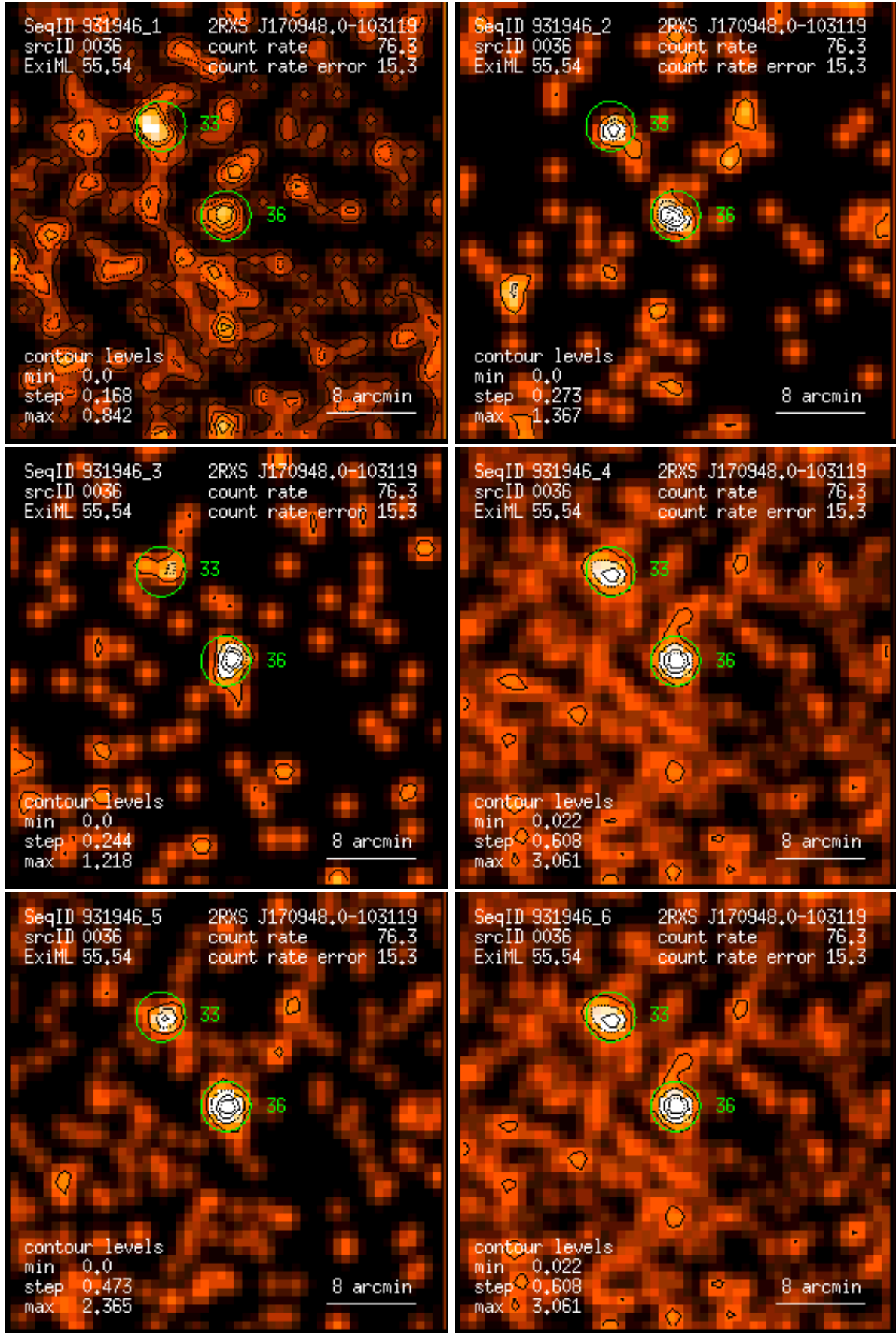
Figure 36: RASS 931946: detection 0036: band rate images, Gaussian filter: (1) PSPC channels 11 – 41, (2) 52 – 90, (3) 91 – 201, (4) 11 – 235, (5) 52 – 201, (6) 11 – 201. Broad band rates in counts/ks. Band rate contour levels in counts/ks/arcmin 2 .
