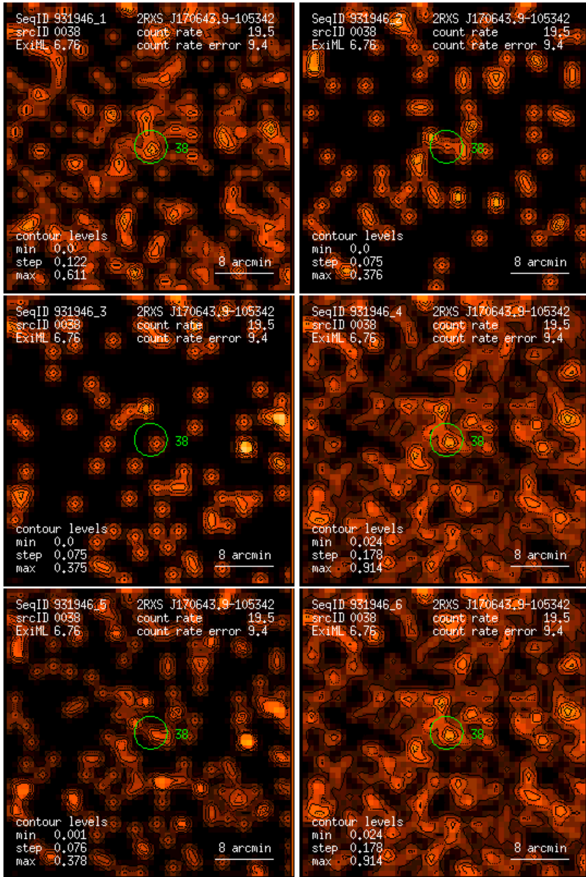
Figure 38: RASS 931946: detection 0038: band rate images, Gaussian filter: (1) PSPC channels 11 – 41, (2) 52 – 90, (3) 91 – 201, (4) 11 – 235, (5) 52 – 201, (6) 11 – 201. Broad band rates in counts/ks. Band rate contour levels in counts/ks/arcmin 2 .
