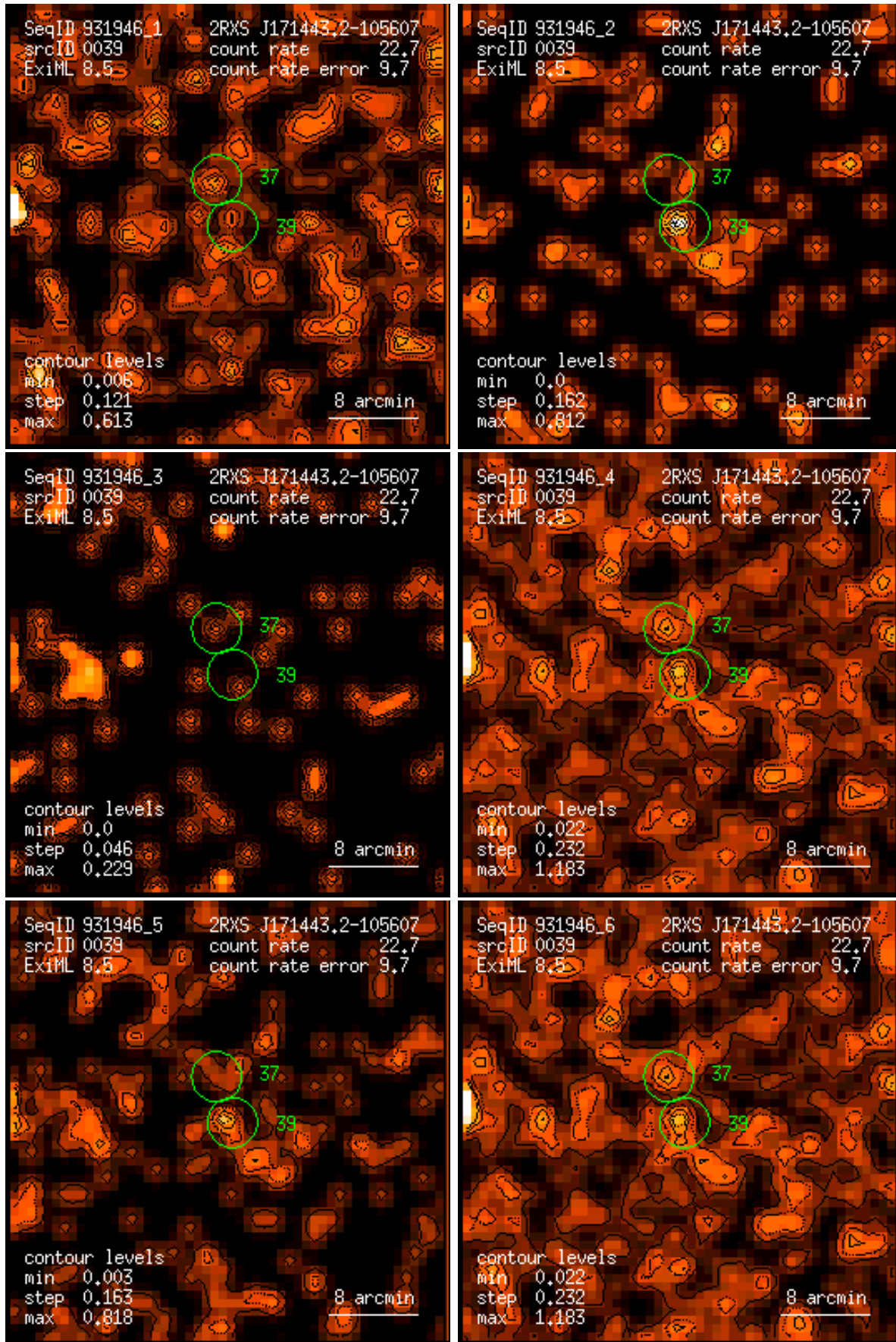
Figure 39: RASS 931946: detection 0039: band rate images, Gaussian filter: (1) PSPC channels 11 – 41, (2) 52 – 90, (3) 91 – 201, (4) 11 – 235, (5) 52 – 201, (6) 11 – 201. Broad band rates in counts/ks. Band rate contour levels in counts/ks/arcmin 2 .
