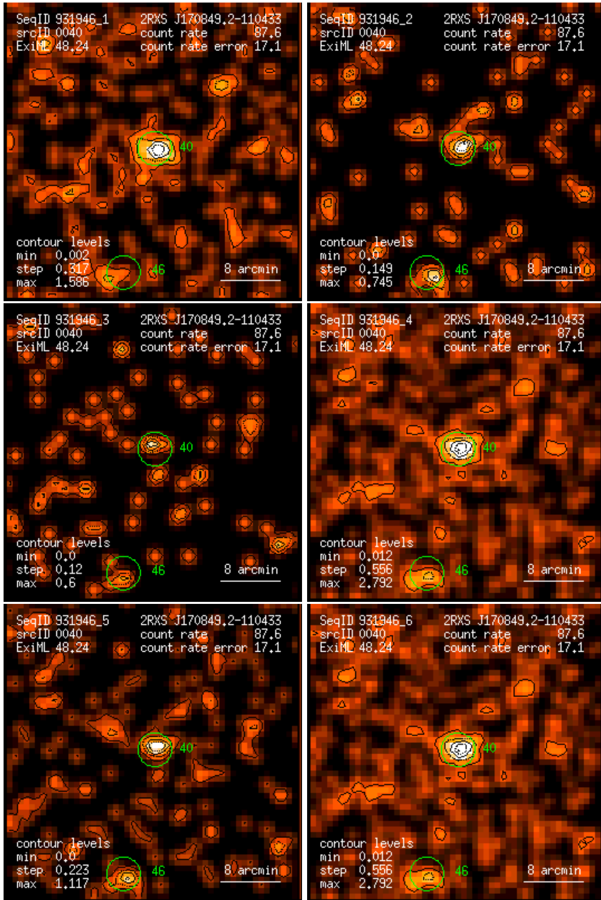
Figure 40: RASS 931946: detection 0040: band rate images, Gaussian filter: (1) PSPC channels 11 – 41, (2) 52 – 90, (3) 91 – 201, (4) 11 – 235, (5) 52 – 201, (6) 11 – 201. Broad band rates in counts/ks. Band rate contour levels in counts/ks/arcmin 2 .
