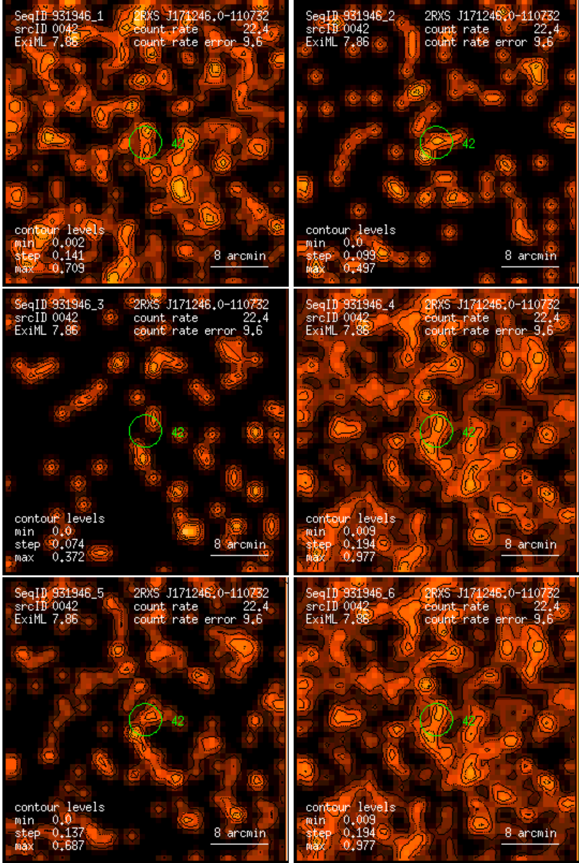
Figure 42: RASS 931946: detection 0042: band rate images, Gaussian filter: (1) PSPC channels 11 – 41, (2) 52 – 90, (3) 91 – 201, (4) 11 – 235, (5) 52 – 201, (6) 11 – 201. Broad band rates in counts/ks. Band rate contour levels in counts/ks/arcmin 2 .
