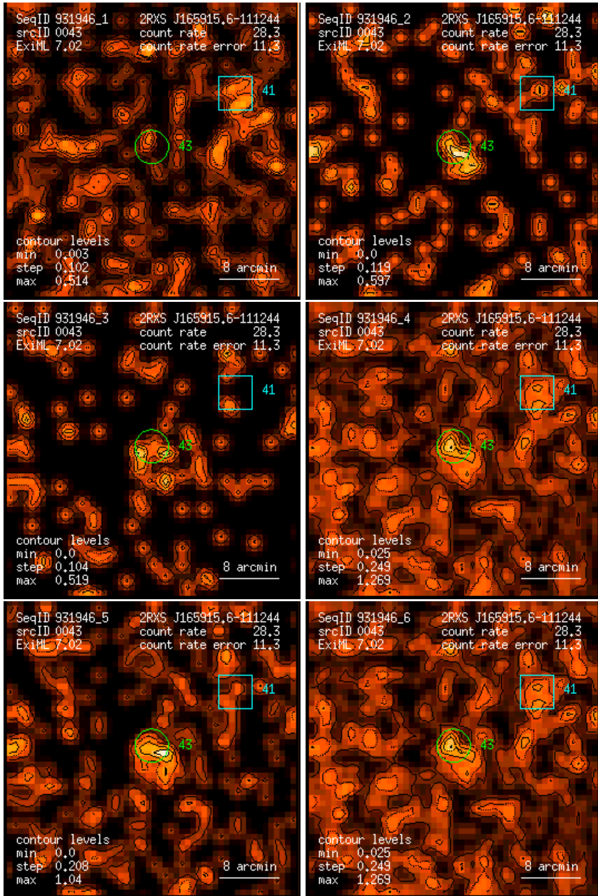
Figure 43: RASS 931946: detection 0043: band rate images, Gaussian filter: (1) PSPC channels 11 – 41, (2) 52 – 90, (3) 91 – 201, (4) 11 – 235, (5) 52 – 201, (6) 11 – 201. Broad band rates in counts/ks. Band rate contour levels in counts/ks/arcmin 2 .
