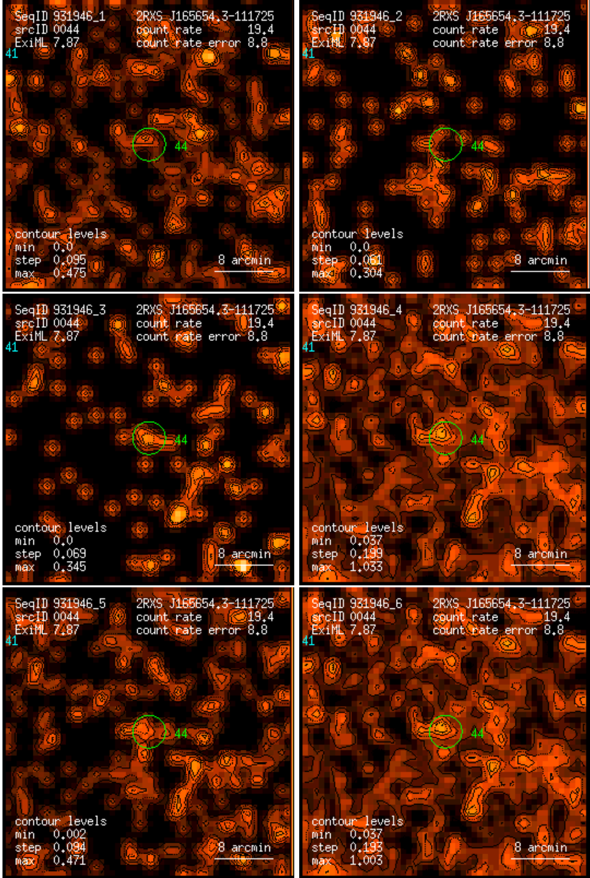
Figure 44: RASS 931946: detection 0044: band rate images, Gaussian filter: (1) PSPC channels 11 – 41, (2) 52 – 90, (3) 91 – 201, (4) 11 – 235, (5) 52 – 201, (6) 11 – 201. Broad band rates in counts/ks. Band rate contour levels in counts/ks/arcmin 2 .
