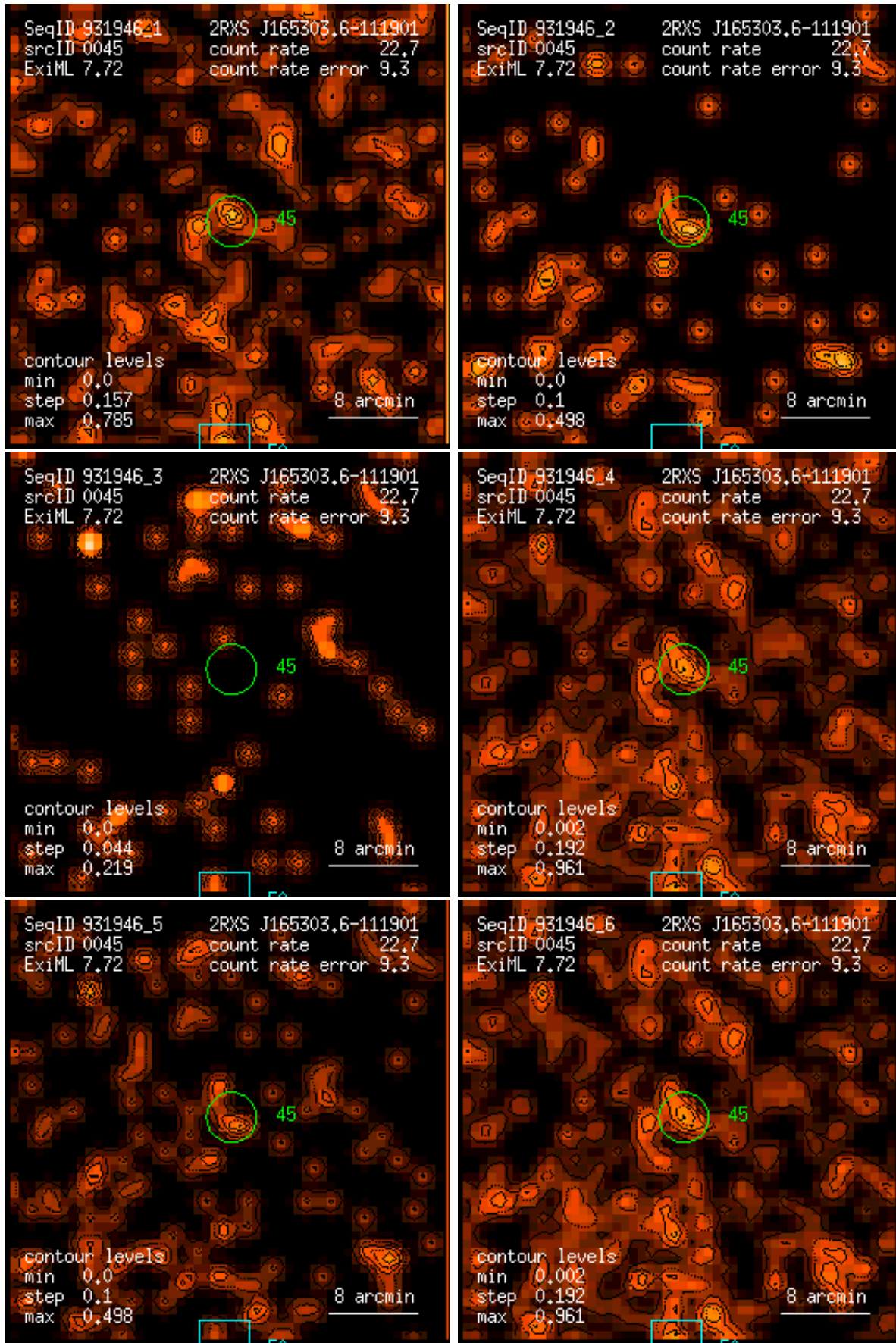
Figure 45: RASS 931946: detection 0045: band rate images, Gaussian filter: (1) PSPC channels 11 – 41, (2) 52 – 90, (3) 91 – 201, (4) 11 – 235, (5) 52 – 201, (6) 11 – 201. Broad band rates in counts/ks. Band rate contour levels in counts/ks/arcmin 2 .
