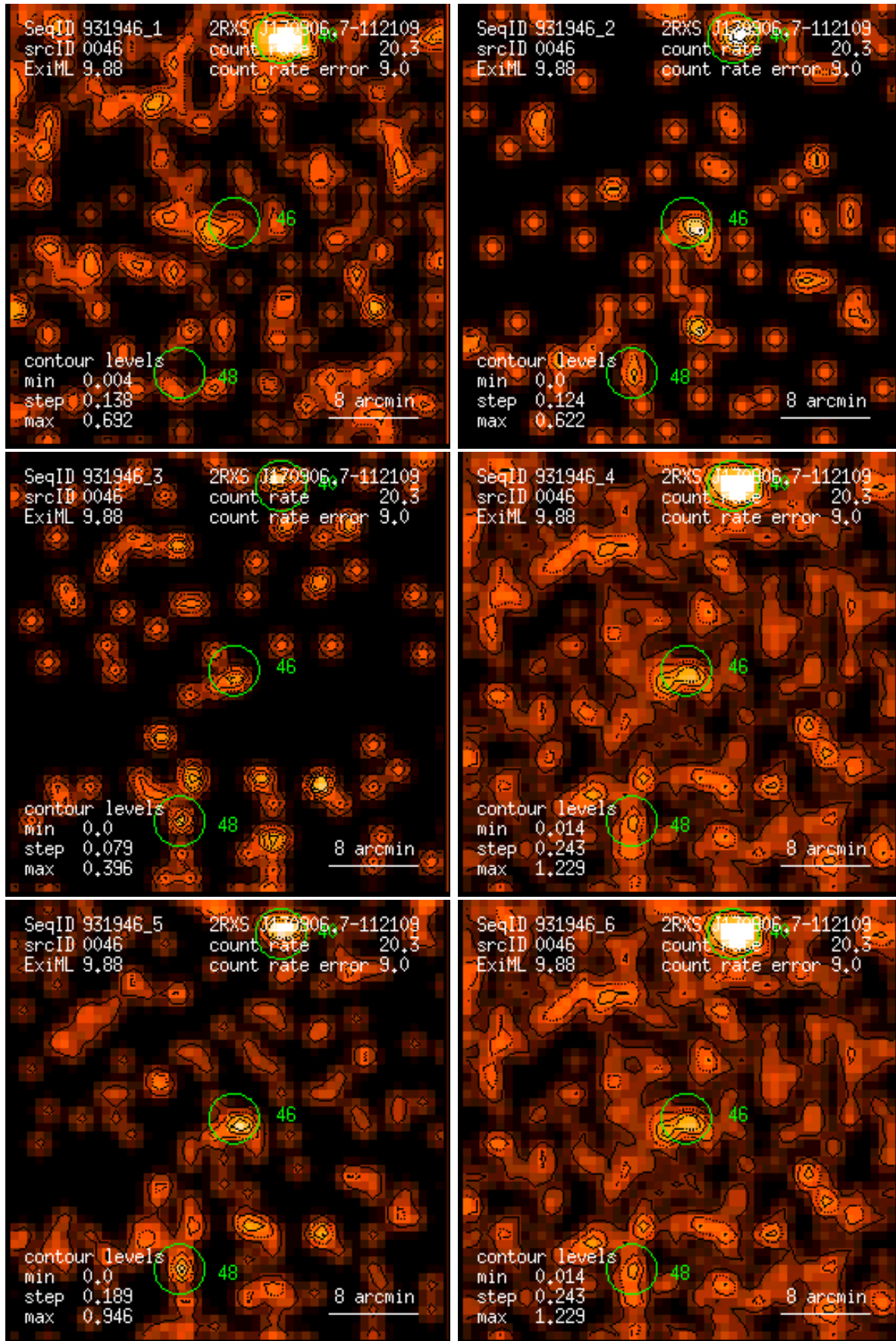
Figure 46: RASS 931946: detection 0046: band rate images, Gaussian filter: (1) PSPC channels 11 – 41, (2) 52 – 90, (3) 91 – 201, (4) 11 – 235, (5) 52 – 201, (6) 11 – 201. Broad band rates in counts/ks. Band rate contour levels in counts/ks/arcmin 2 .
