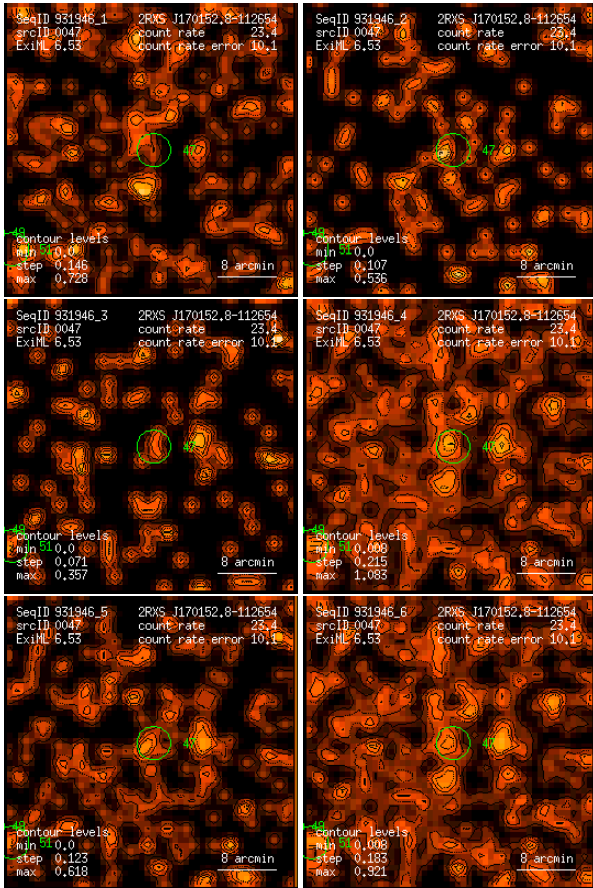
Figure 47: RASS 931946: detection 0047: band rate images, Gaussian filter: (1) PSPC channels 11 – 41, (2) 52 – 90, (3) 91 – 201, (4) 11 – 235, (5) 52 – 201, (6) 11 – 201. Broad band rates in counts/ks. Band rate contour levels in counts/ks/arcmin 2 .
