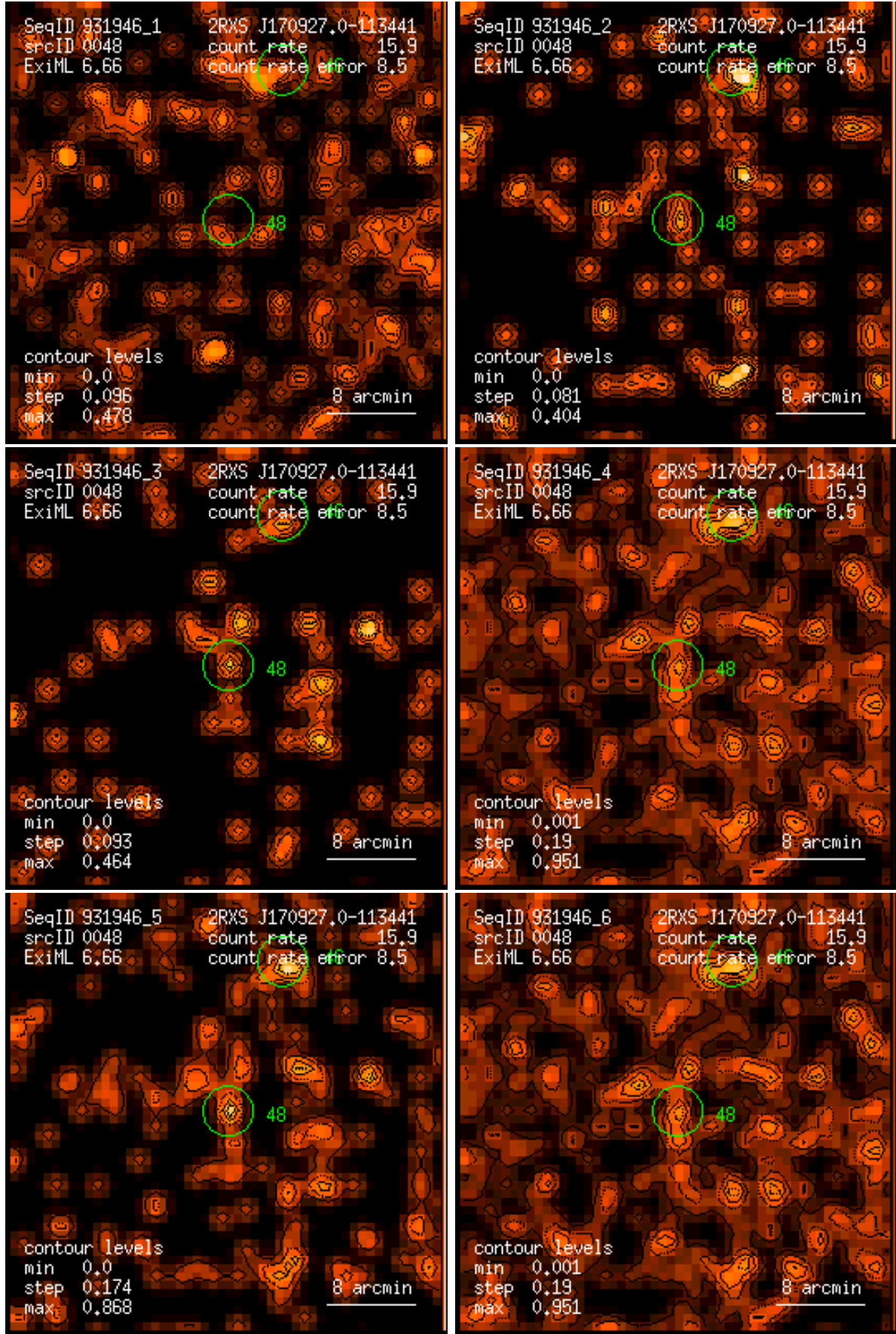
Figure 48: RASS 931946: detection 0048: band rate images, Gaussian filter: (1) PSPC channels 11 – 41, (2) 52 – 90, (3) 91 – 201, (4) 11 – 235, (5) 52 – 201, (6) 11 – 201. Broad band rates in counts/ks. Band rate contour levels in counts/ks/arcmin 2 .
