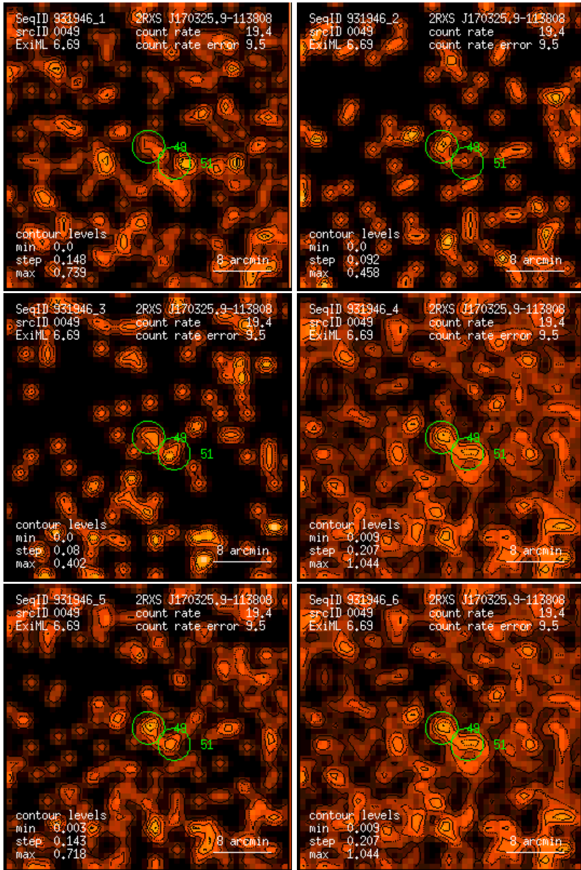
Figure 49: RASS 931946: detection 0049: band rate images, Gaussian filter: (1) PSPC channels 11 – 41, (2) 52 – 90, (3) 91 – 201, (4) 11 – 235, (5) 52 – 201, (6) 11 – 201. Broad band rates in counts/ks. Band rate contour levels in counts/ks/arcmin 2 .
