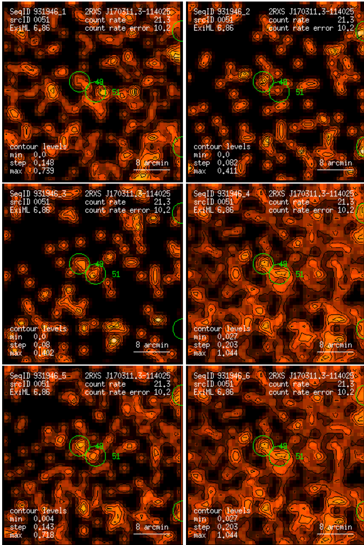
Figure 51: RASS 931946: detection 0051: band rate images, Gaussian filter: (1) PSPC channels 11 – 41, (2) 52 – 90, (3) 91 – 201, (4) 11 – 235, (5) 52 – 201, (6) 11 – 201. Broad band rates in counts/ks. Band rate contour levels in counts/ks/arcmin 2 .
