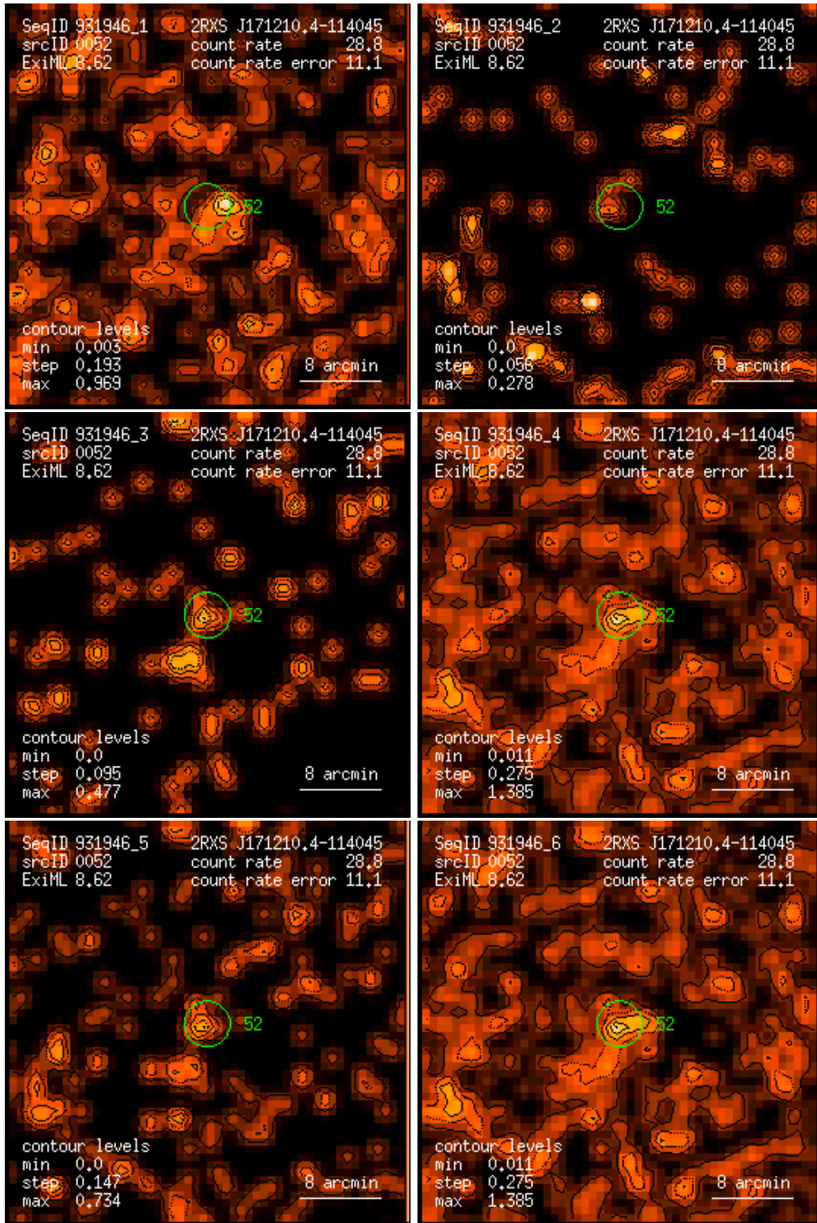
Figure 52: RASS 931946: detection 0052: band rate images, Gaussian filter: (1) PSPC channels 11 – 41, (2) 52 – 90, (3) 91 – 201, (4) 11 – 235, (5) 52 – 201, (6) 11 – 201. Broad band rates in counts/ks. Band rate contour levels in counts/ks/arcmin 2 .
