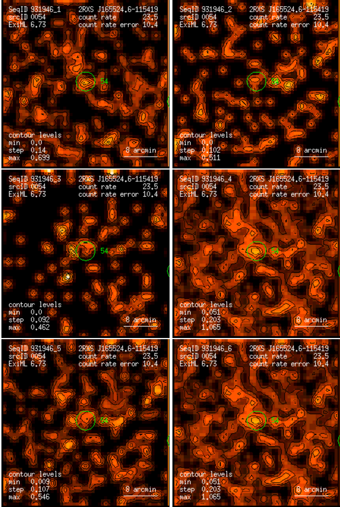
Figure 54: RASS 931946: detection 0054: band rate images, Gaussian filter: (1) PSPC channels 11 – 41, (2) 52 – 90, (3) 91 – 201, (4) 11 – 235, (5) 52 – 201, (6) 11 – 201. Broad band rates in counts/ks. Band rate contour levels in counts/ks/arcmin 2 .
