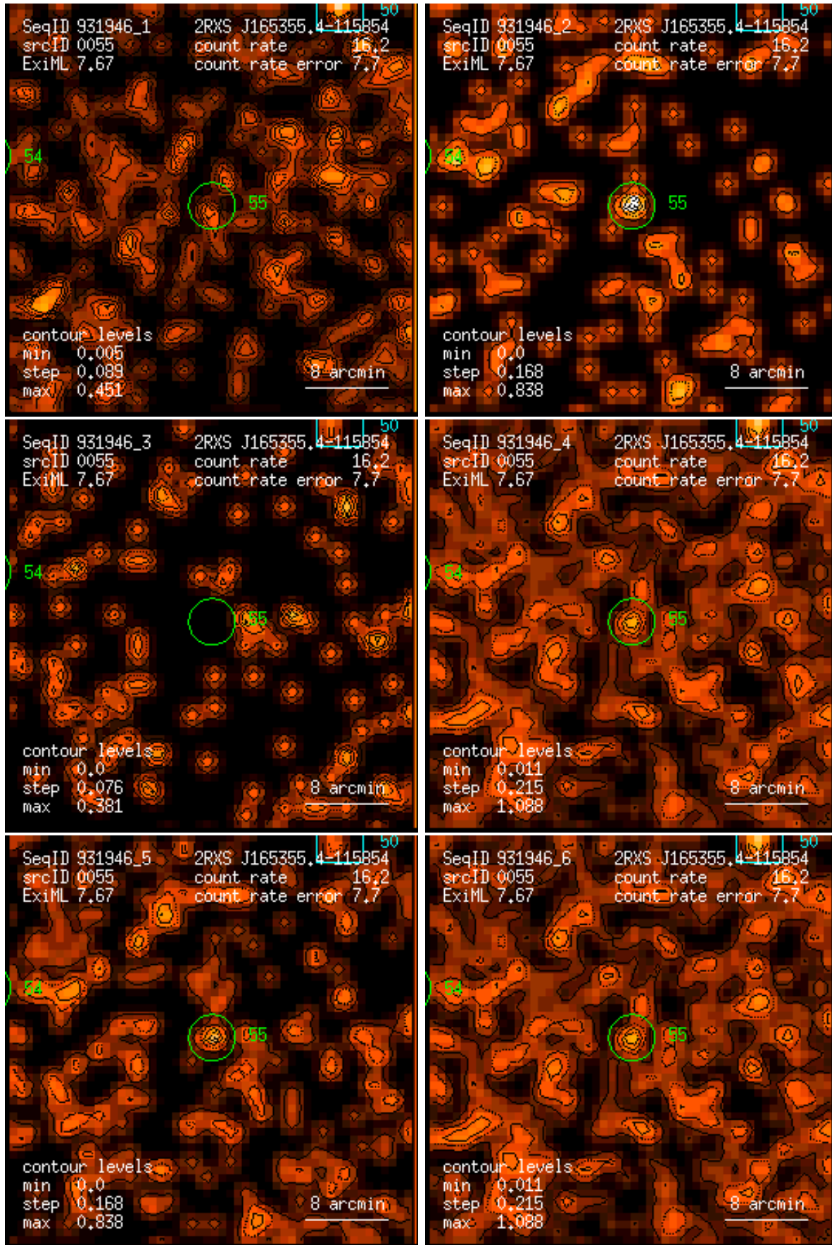
Figure 55: RASS 931946: detection 0055: band rate images, Gaussian filter: (1) PSPC channels 11 – 41, (2) 52 – 90, (3) 91 – 201, (4) 11 – 235, (5) 52 – 201, (6) 11 – 201. Broad band rates in counts/ks. Band rate contour levels in counts/ks/arcmin 2 .
