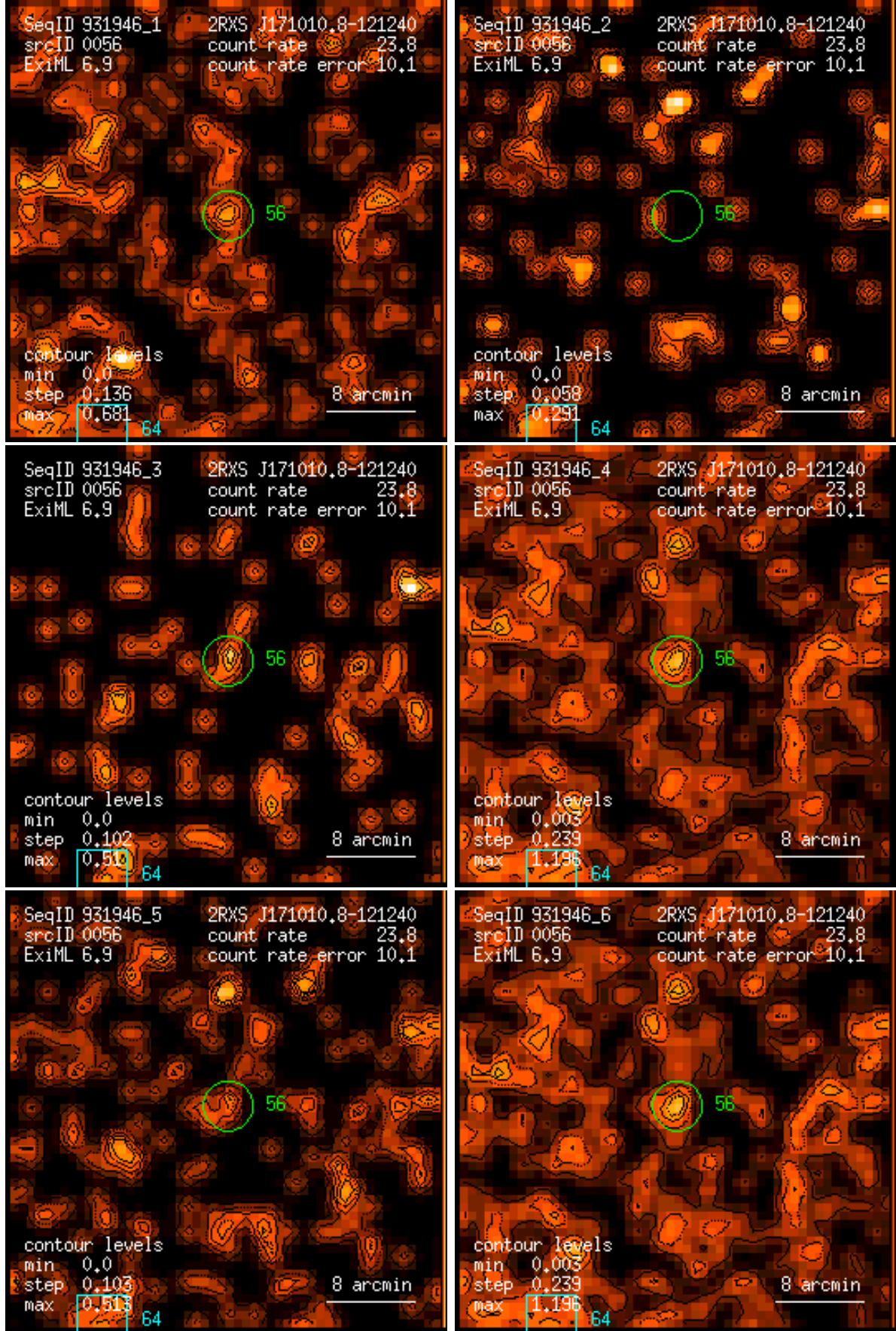
Figure 56: RASS 931946: detection 0056: band rate images, Gaussian filter: (1) PSPC channels 11 – 41, (2) 52 – 90, (3) 91 – 201, (4) 11 – 235, (5) 52 – 201, (6) 11 – 201. Broad band rates in counts/ks. Band rate contour levels in counts/ks/arcmin 2 .
