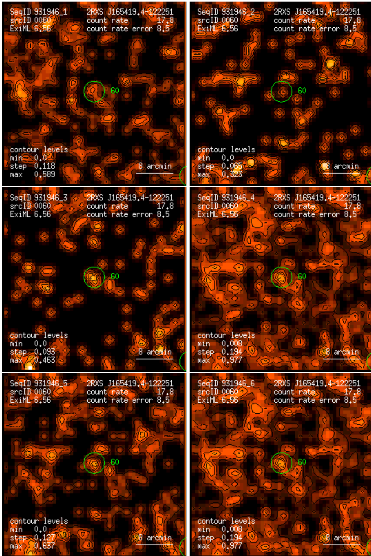
Figure 60: RASS 931946: detection 0060: band rate images, Gaussian filter: (1) PSPC channels 11 – 41, (2) 52 – 90, (3) 91 – 201, (4) 11 – 235, (5) 52 – 201, (6) 11 – 201. Broad band rates in counts/ks. Band rate contour levels in counts/ks/arcmin 2 .
