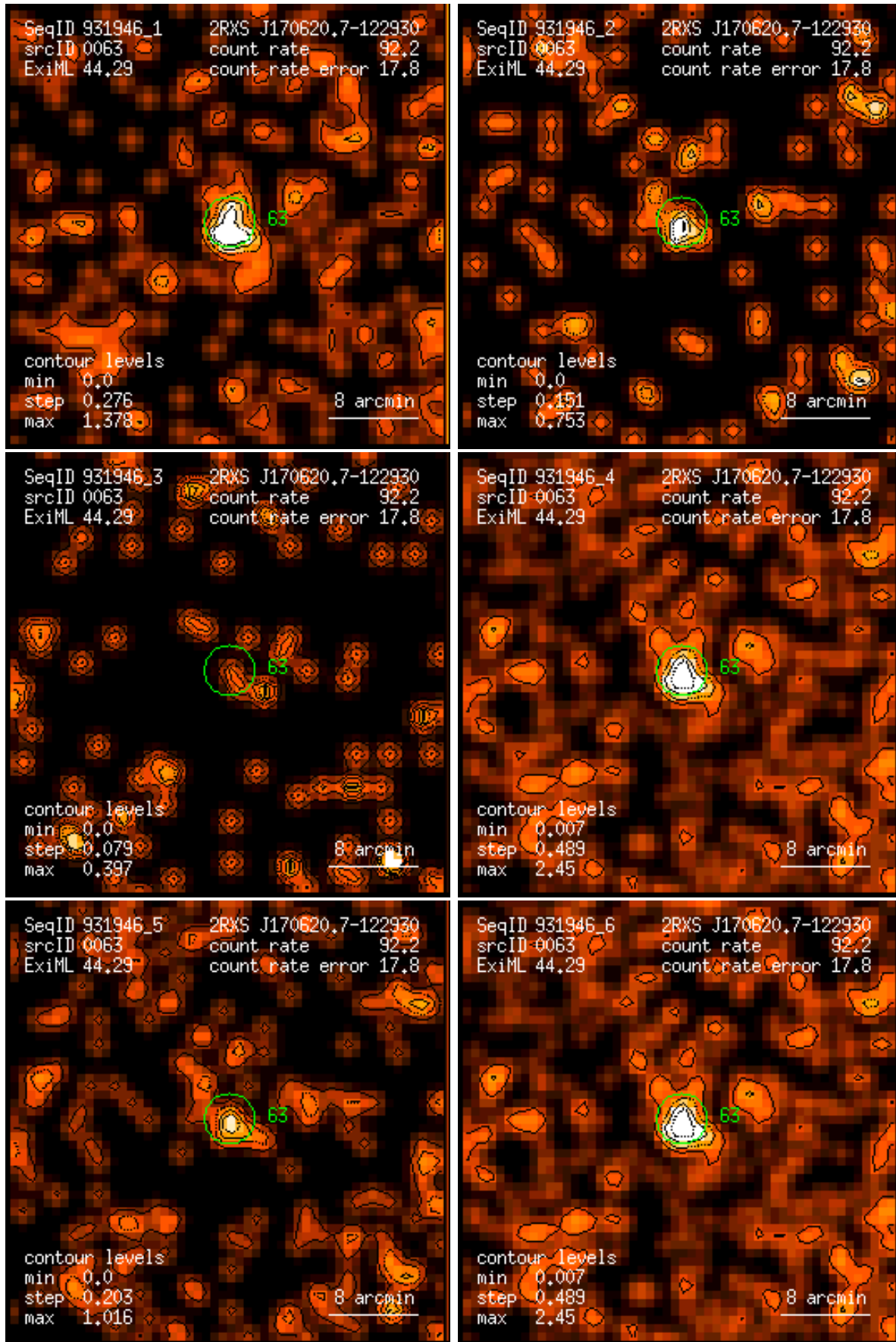
Figure 63: RASS 931946: detection 0063: band rate images, Gaussian filter: (1) PSPC channels 11 – 41, (2) 52 – 90, (3) 91 – 201, (4) 11 – 235, (5) 52 – 201, (6) 11 – 201. Broad band rates in counts/ks. Band rate contour levels in counts/ks/arcmin 2 .
