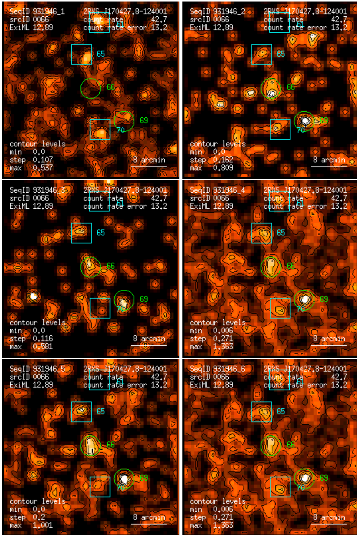
Figure 66: RASS 931946: detection 0066: band rate images, Gaussian filter: (1) PSPC channels 11 – 41, (2) 52 – 90, (3) 91 – 201, (4) 11 – 235, (5) 52 – 201, (6) 11 – 201. Broad band rates in counts/ks. Band rate contour levels in counts/ks/arcmin 2 .
