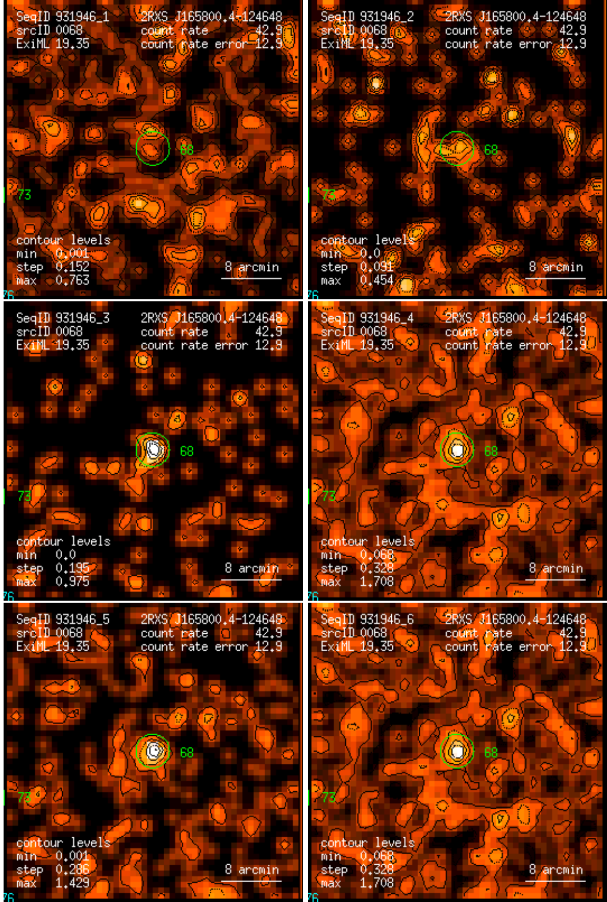
Figure 68: RASS 931946: detection 0068: band rate images, Gaussian filter: (1) PSPC channels 11 – 41, (2) 52 – 90, (3) 91 – 201, (4) 11 – 235, (5) 52 – 201, (6) 11 – 201. Broad band rates in counts/ks. Band rate contour levels in counts/ks/arcmin 2 .
