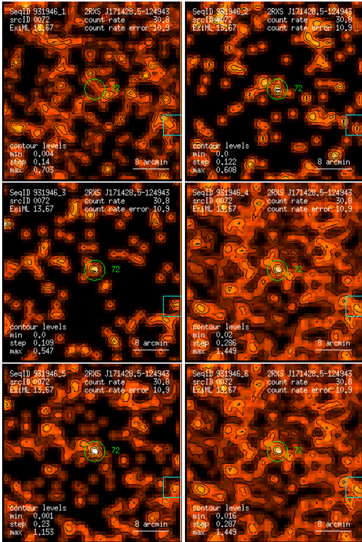
Figure 72: RASS 931946: detection 0072: band rate images, Gaussian filter: (1) PSPC channels 11 – 41, (2) 52 – 90, (3) 91 – 201, (4) 11 – 235, (5) 52 – 201, (6) 11 – 201. Broad band rates in counts/ks. Band rate contour levels in counts/ks/arcmin 2 .
