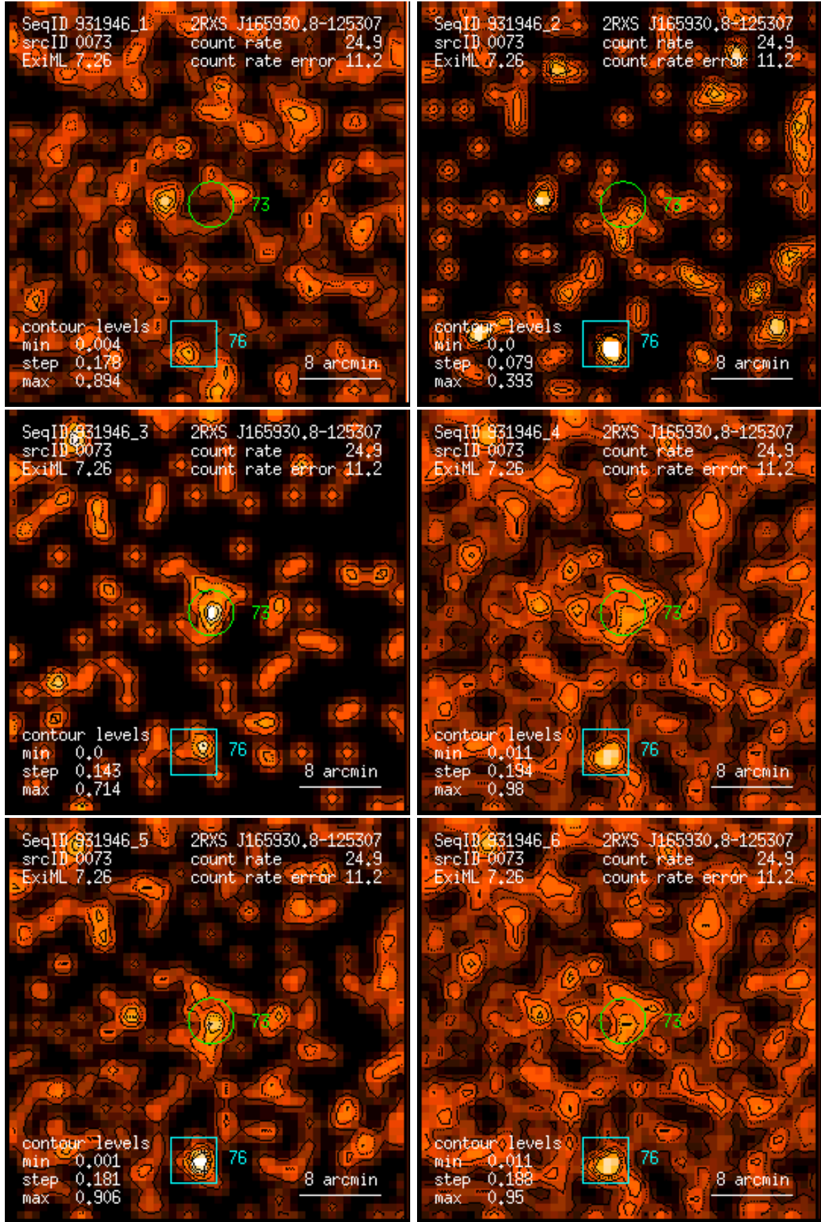
Figure 73: RASS 931946: detection 0073: band rate images, Gaussian filter: (1) PSPC channels 11 – 41, (2) 52 – 90, (3) 91 – 201, (4) 11 – 235, (5) 52 – 201, (6) 11 – 201. Broad band rates in counts/ks. Band rate contour levels in counts/ks/arcmin 2 .
