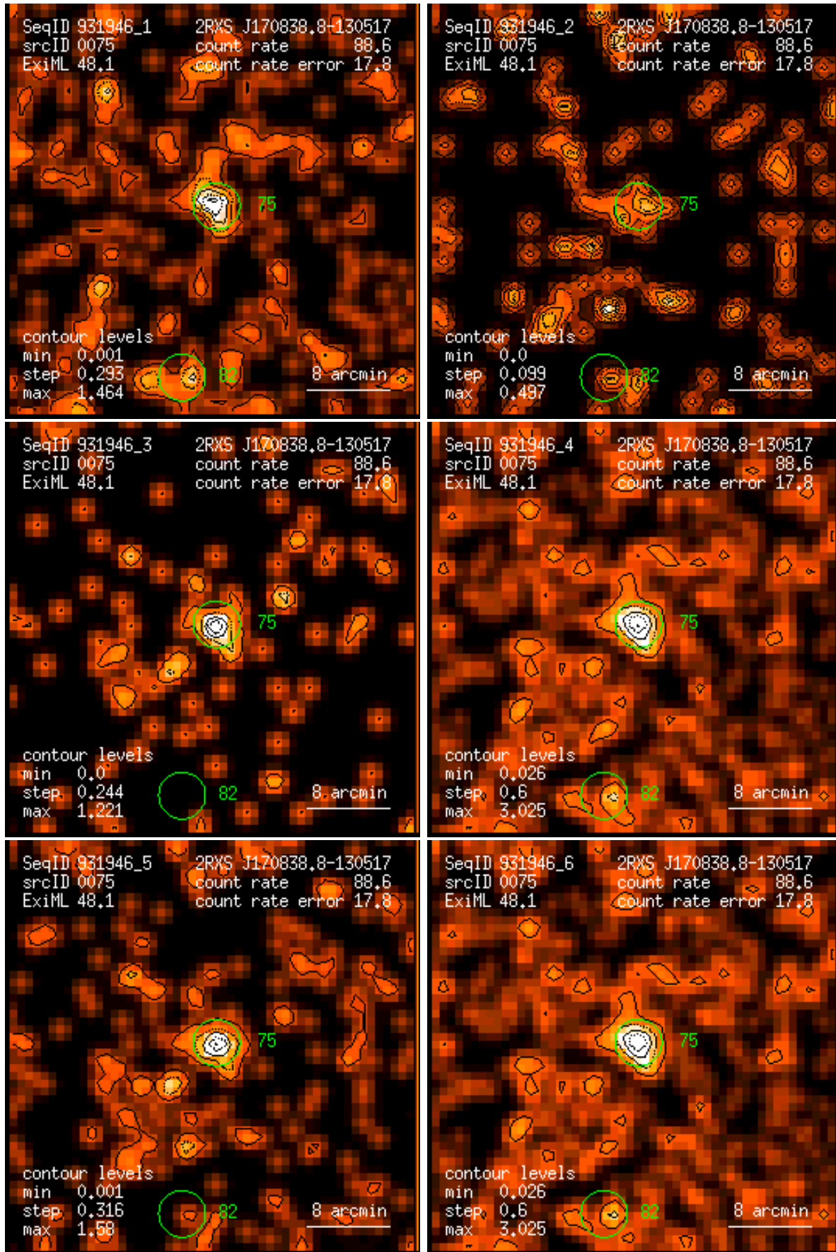
Figure 75: RASS 931946: detection 0075: band rate images, Gaussian filter: (1) PSPC channels 11 – 41, (2) 52 – 90, (3) 91 – 201, (4) 11 – 235, (5) 52 – 201, (6) 11 – 201. Broad band rates in counts/ks. Band rate contour levels in counts/ks/arcmin 2 .
