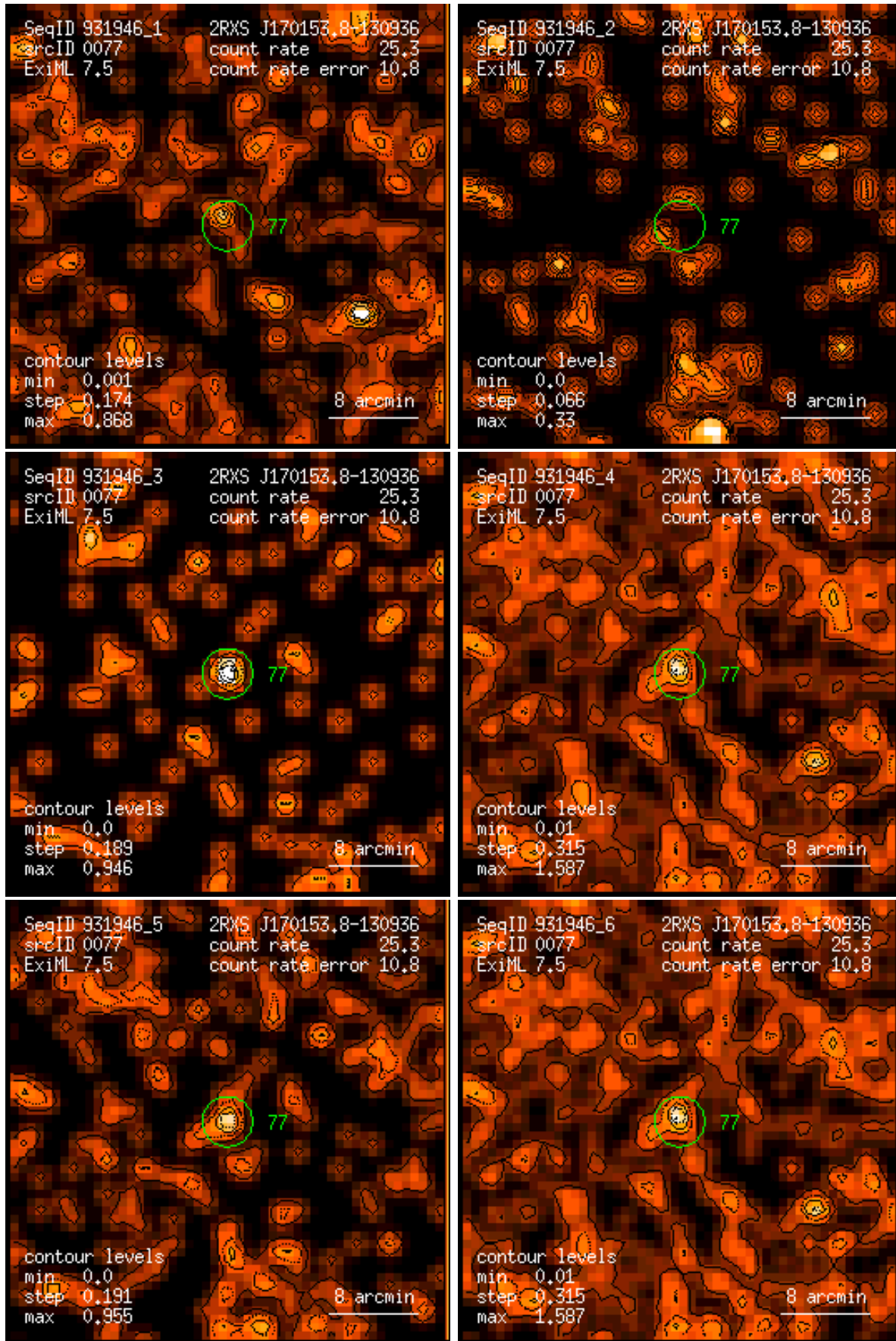
Figure 77: RASS 931946: detection 0077: band rate images, Gaussian filter: (1) PSPC channels 11 – 41, (2) 52 – 90, (3) 91 – 201, (4) 11 – 235, (5) 52 – 201, (6) 11 – 201. Broad band rates in counts/ks. Band rate contour levels in counts/ks/arcmin 2 .
