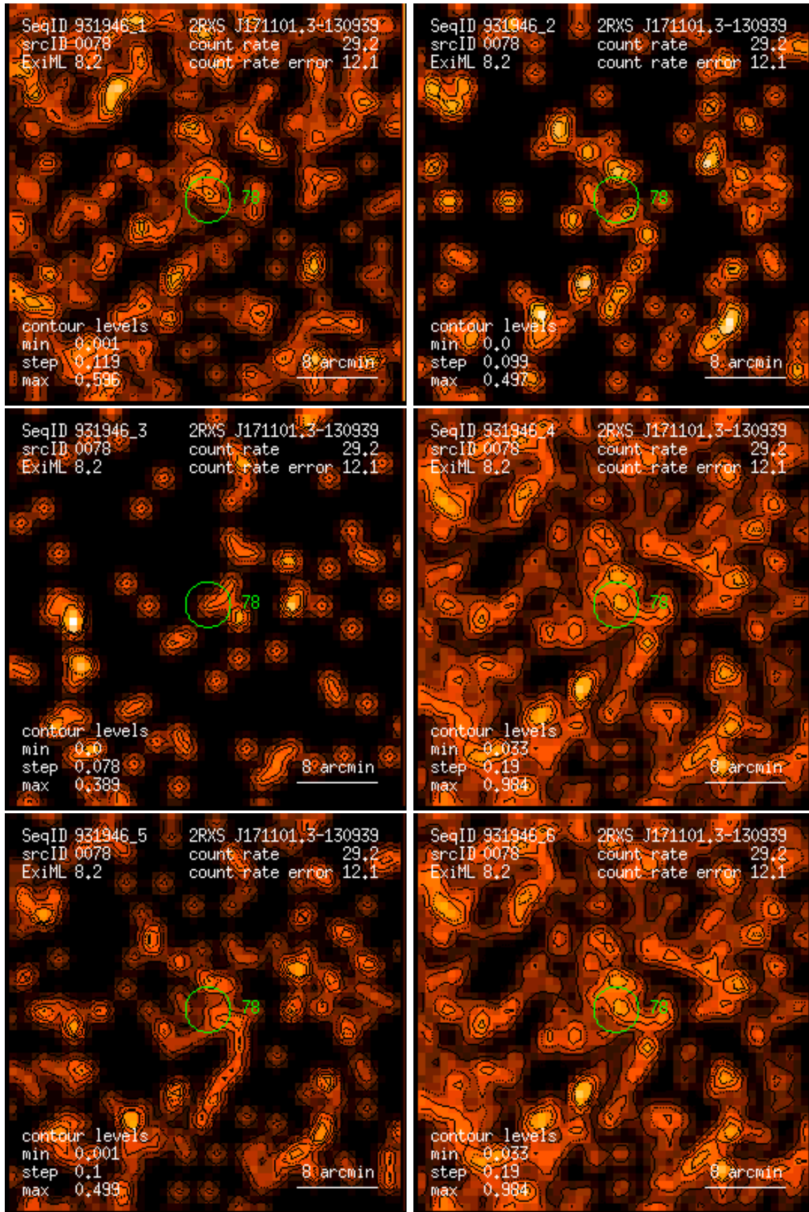
Figure 78: RASS 931946: detection 0078: band rate images, Gaussian filter: (1) PSPC channels 11 – 41, (2) 52 – 90, (3) 91 – 201, (4) 11 – 235, (5) 52 – 201, (6) 11 – 201. Broad band rates in counts/ks. Band rate contour levels in counts/ks/arcmin 2 .
